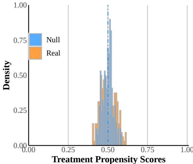
Balance Permutation Test
