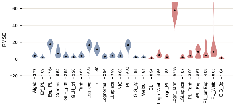
b Function performance, RMSE
