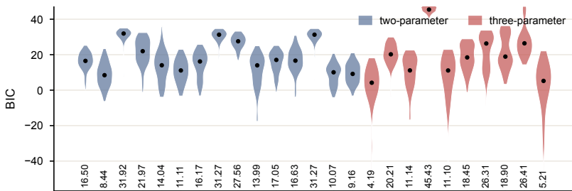
a Function performance, BIC
