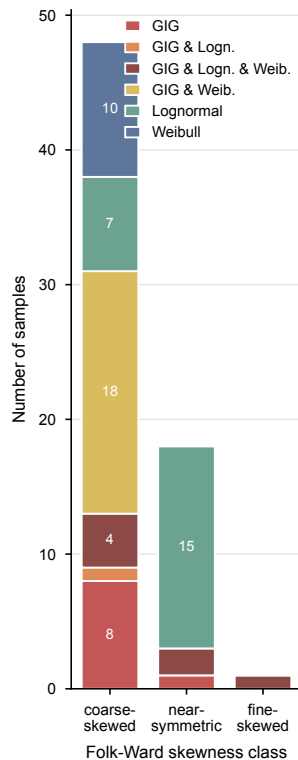
c Best-fit set by skewness class
