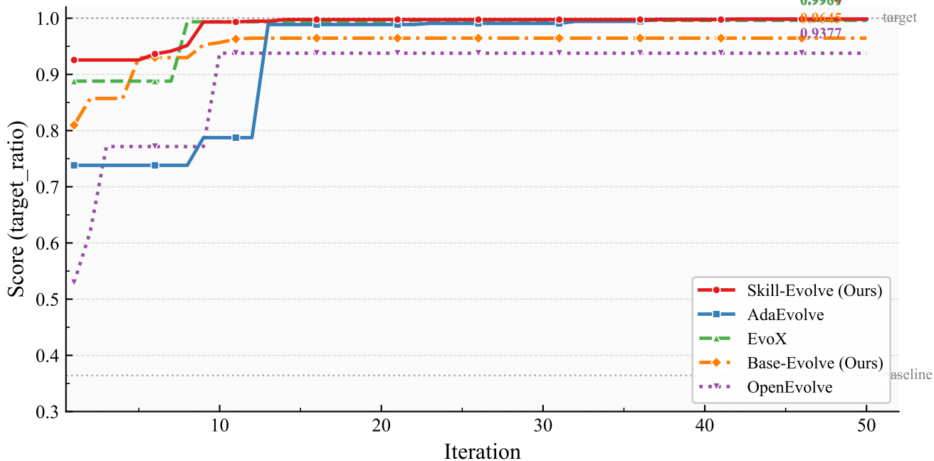
Circle Packing (n=26) — Best Run per Framework — 50 Iterations
