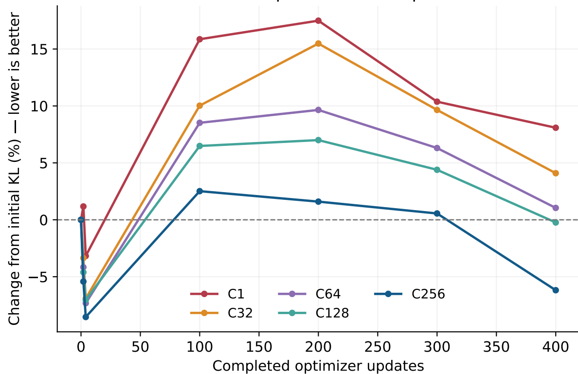
Held-out prefill KL vs. step 0
