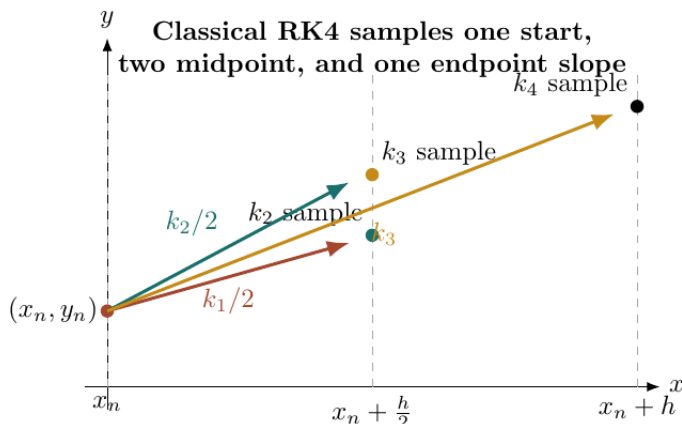
Figure 1: Schematic of the four classical RK4 stage locations
