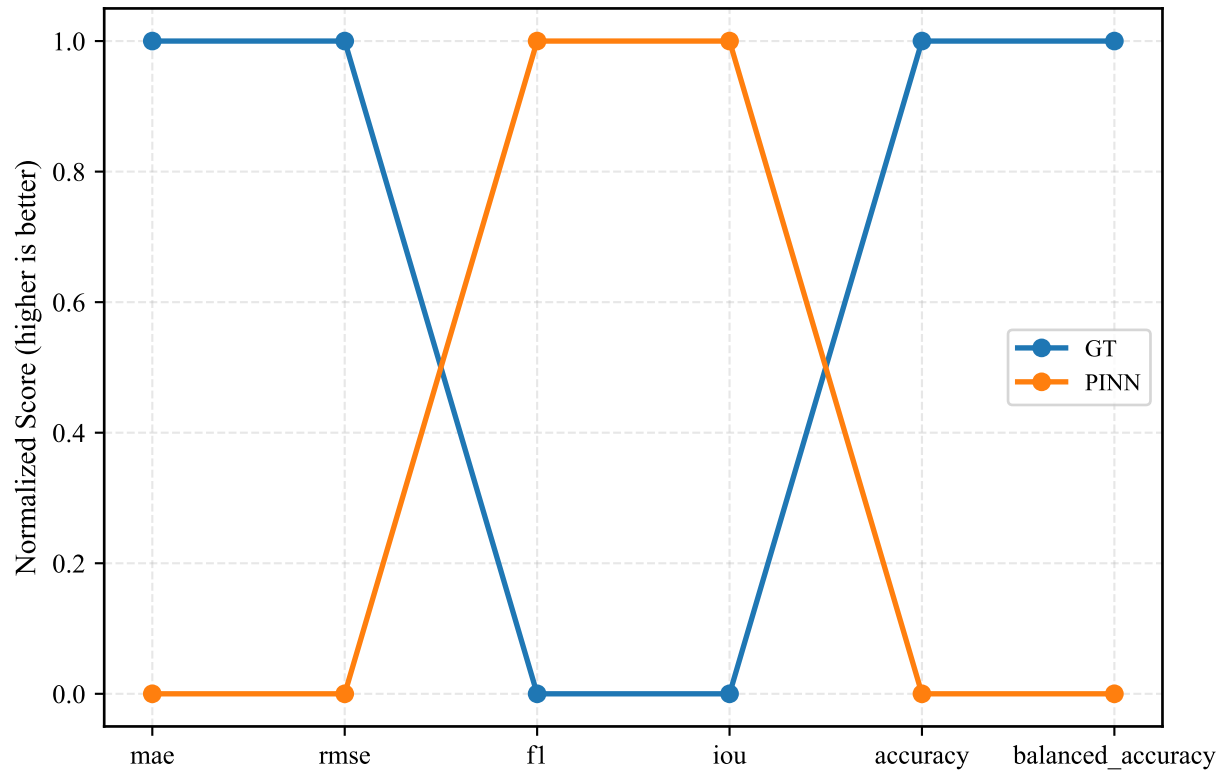
Direction-Aware Normalized Comparison
