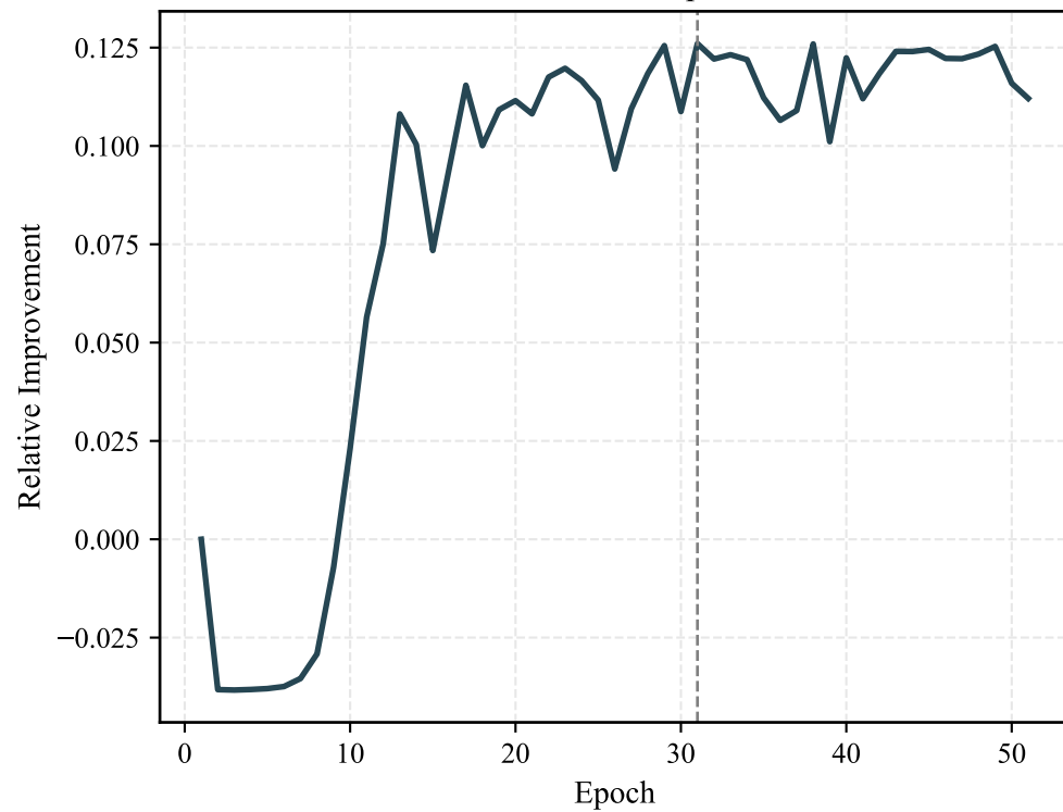
LSTM Validation Improvement
