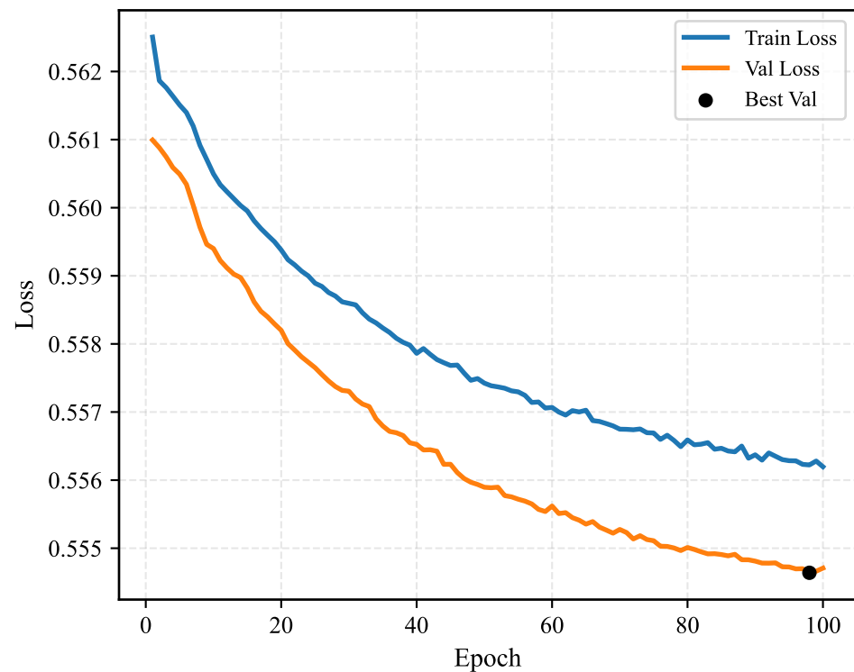
PINN Generalization Gap
