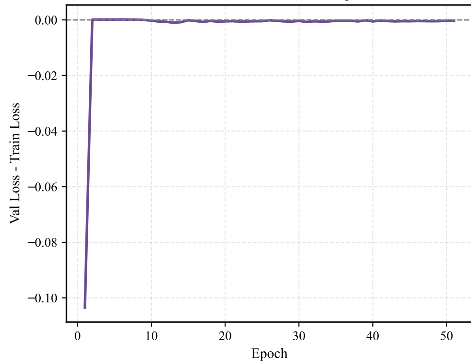
LSTM Generalization Gap
