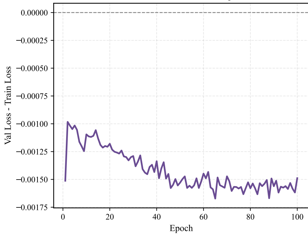
PINN Generalization Gap
