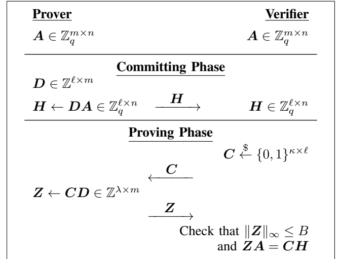
Figure 2: SIS Hash (Commitment) and Proof of Knowledge for Its Preimage [10]. For a purported infinity-norm bound \beta of D , we set B \geq \ell \cdot \beta .
