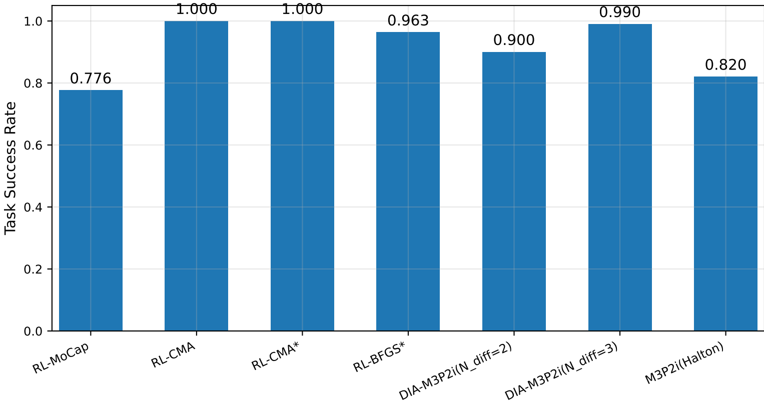
FetchPickDynamic-LiftedObstaclesMaze
