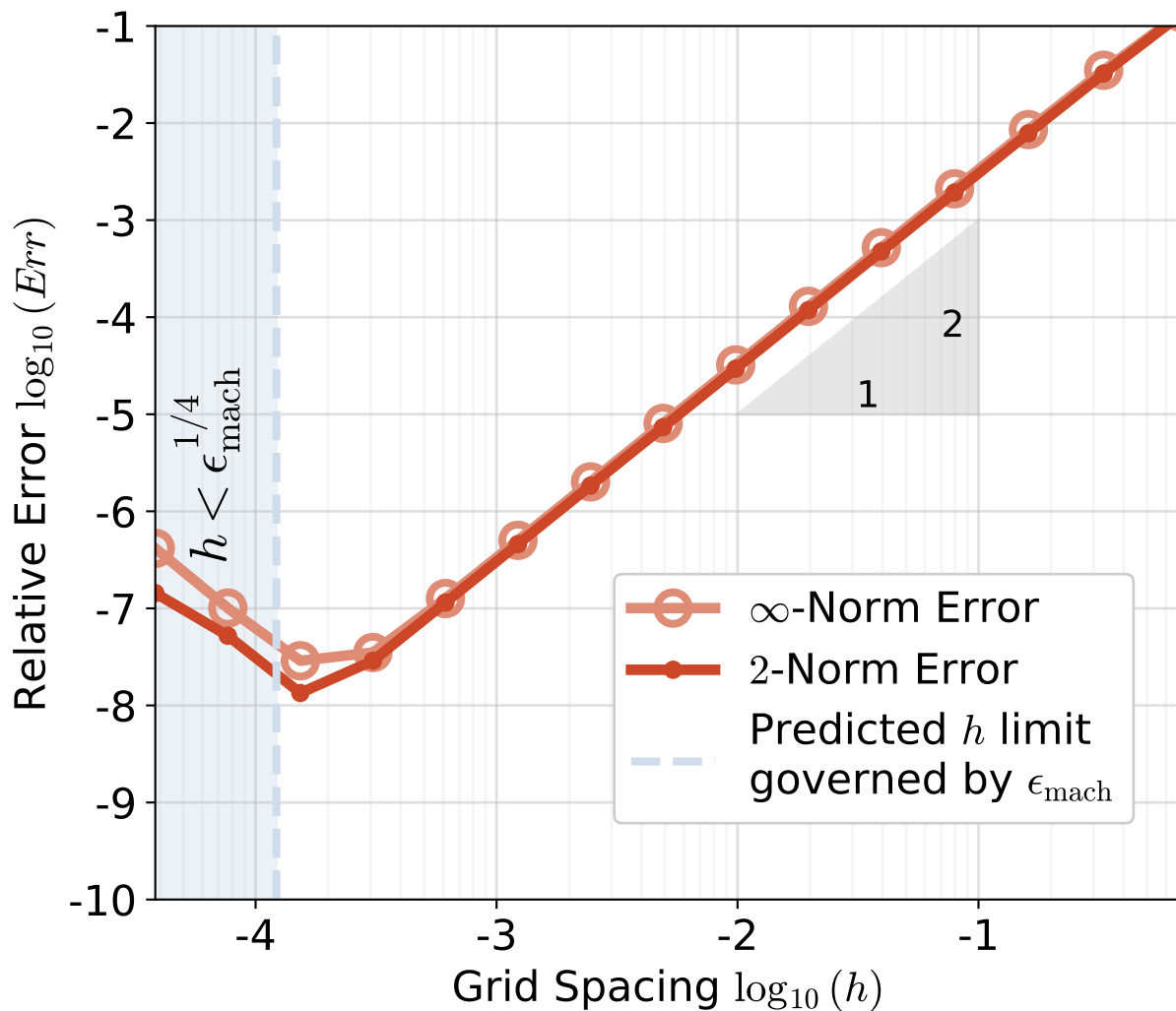
Figure 2.2: p -norm convergence for p \in \{2, \infty\} of the second-derivative approximation.
