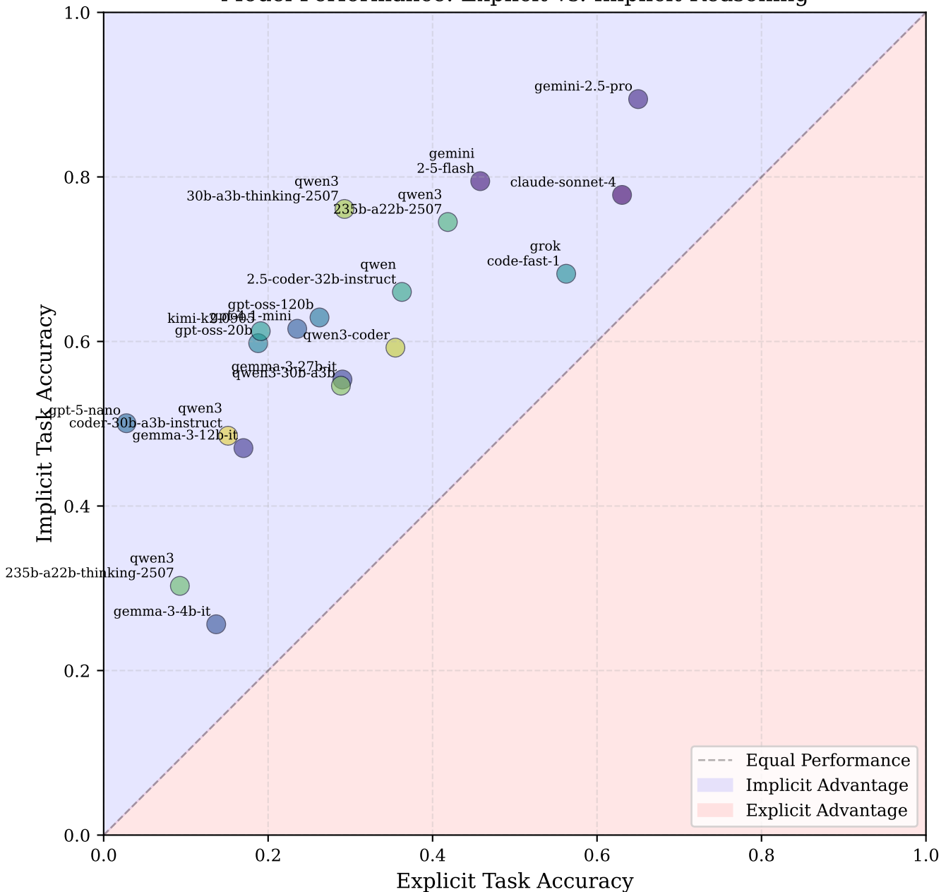
Model Performance: Explicit vs. Implicit Reasoning
