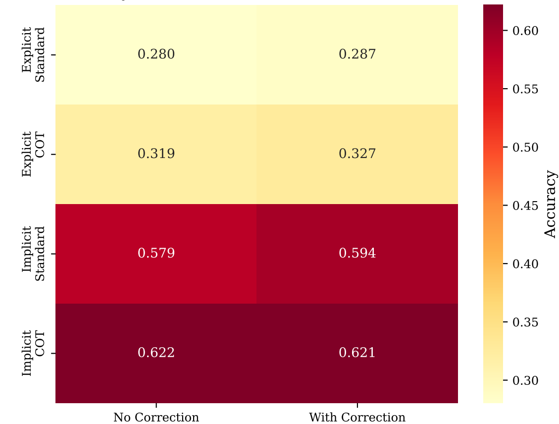
Three-Way Interaction: Context × Method × Correction
