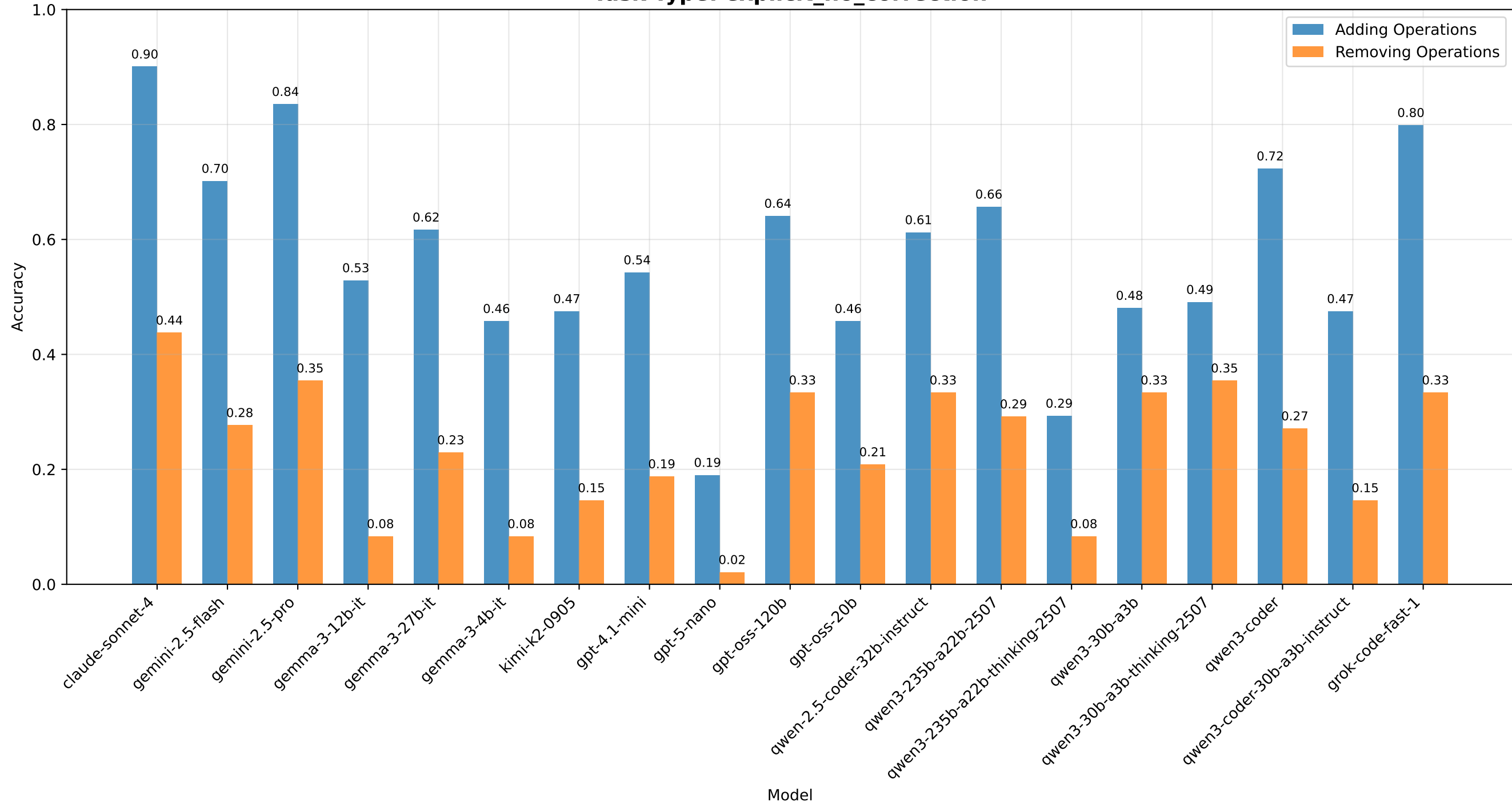
Accuracy Comparison: Adding vs Removing Operations Task Type: explicit_no_correction
