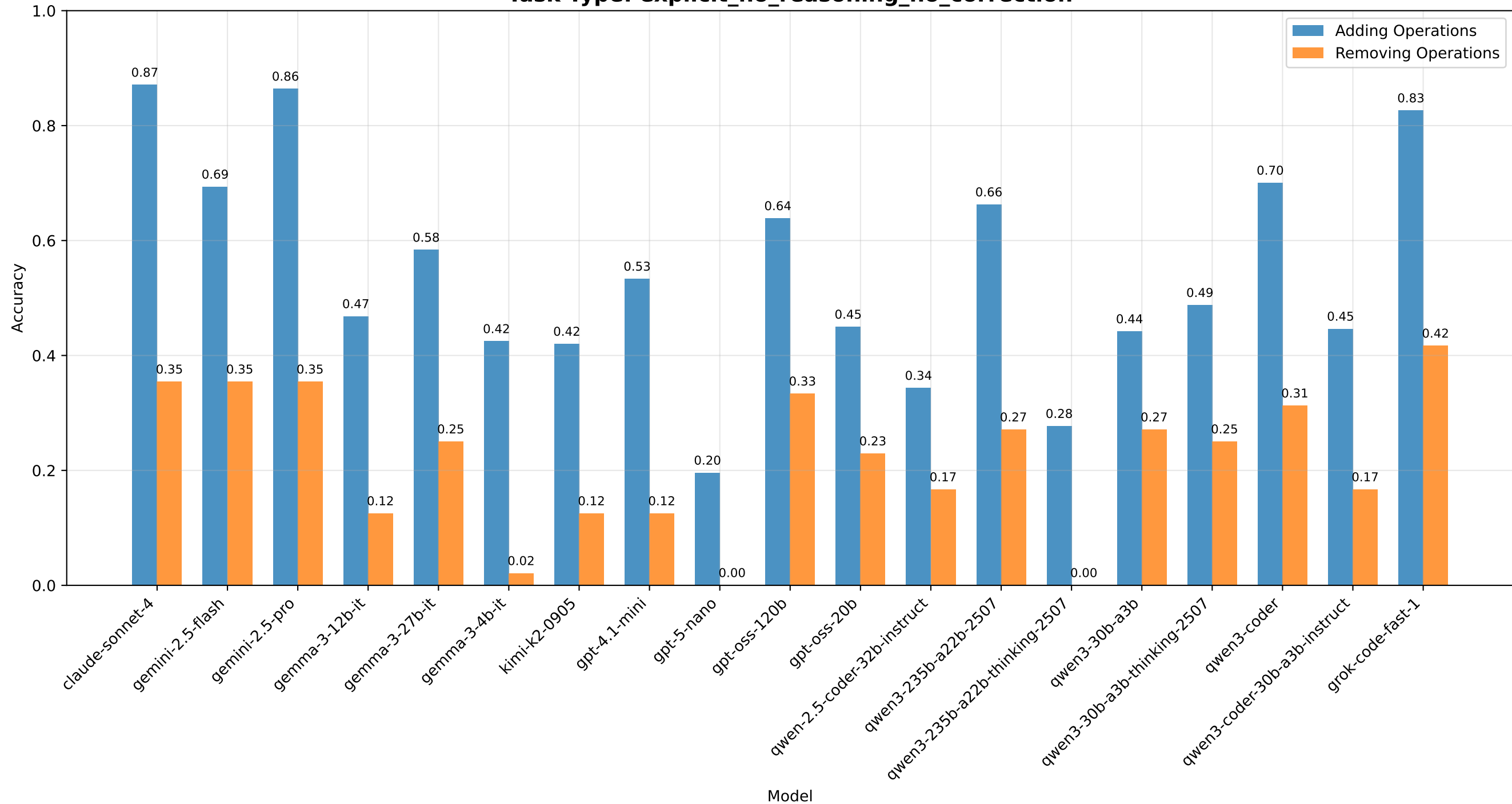
Accuracy Comparison: Adding vs Removing Operations Task Type: explicit_no_reasoning_no_correction
