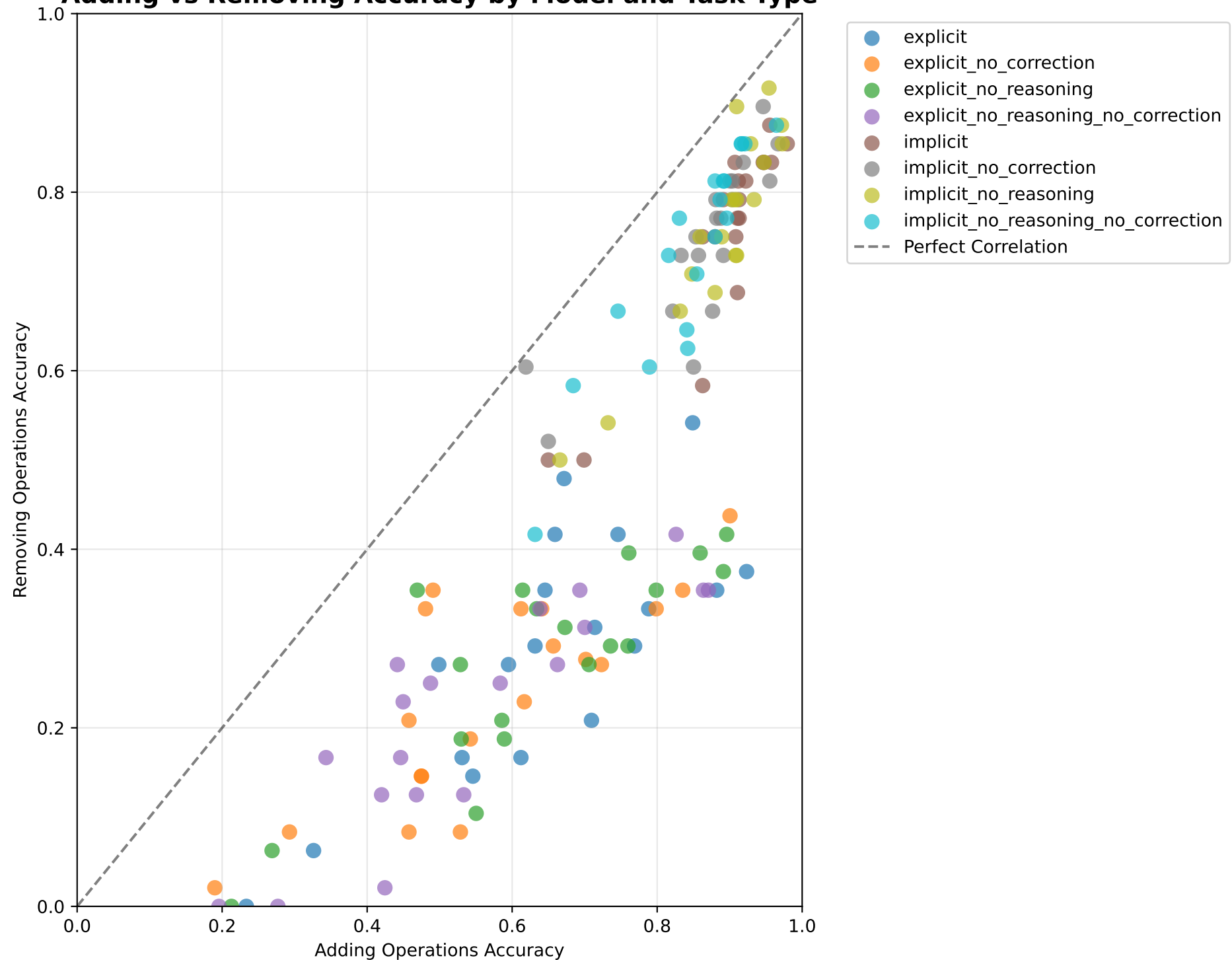
Adding vs Removing Accuracy by Model and Task Type
