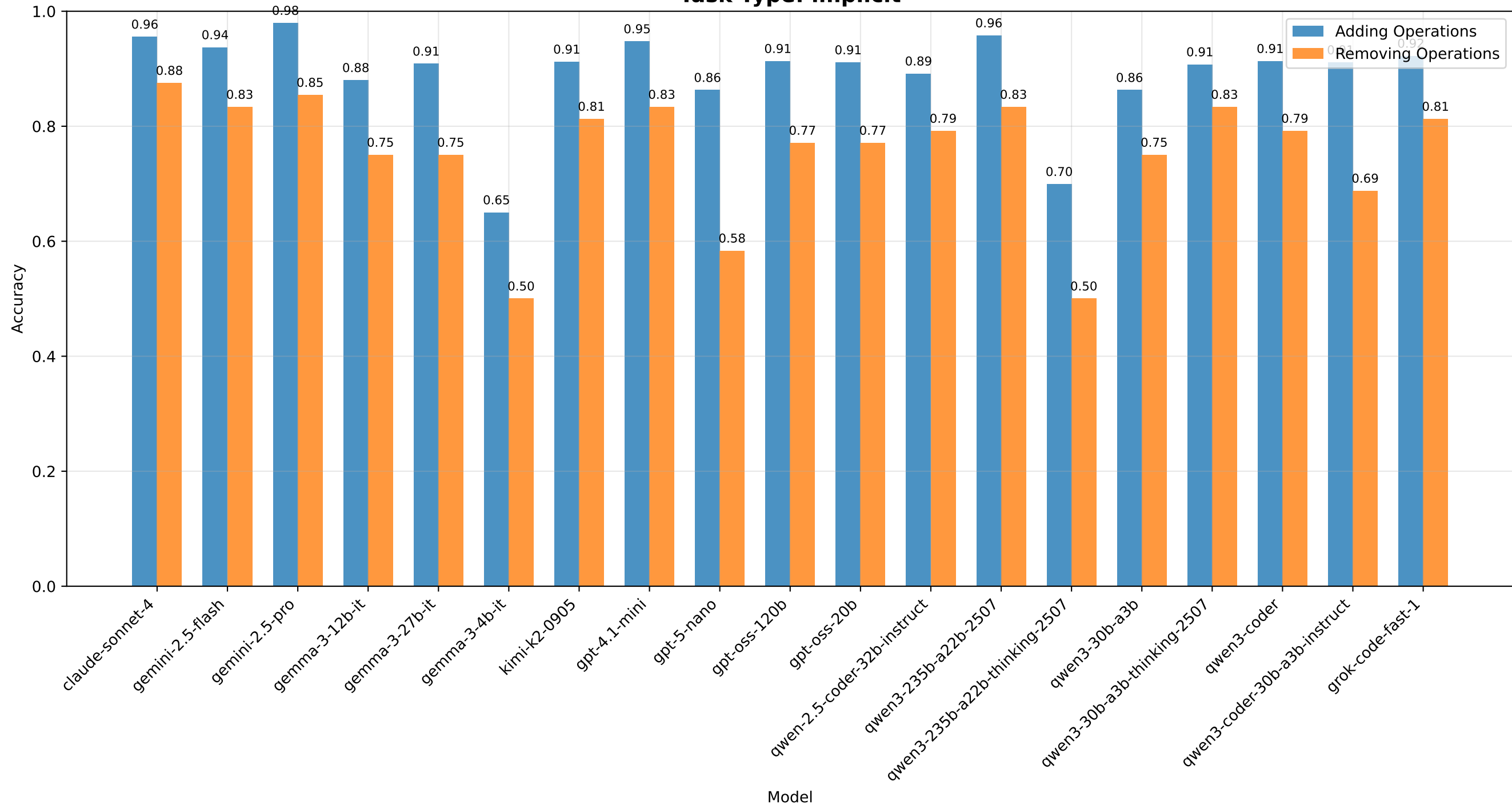
Accuracy Comparison: Adding vs Removing Operations Task Type: implicit
