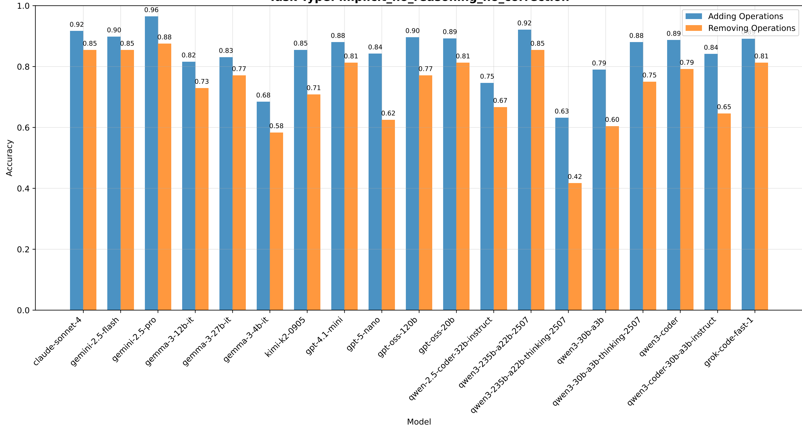
Accuracy Comparison: Adding vs Removing Operations Task Type: implicit_no_reasoning_no_correction
