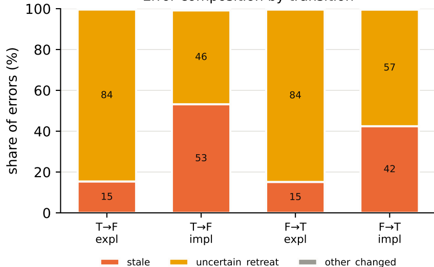
Error composition by transition
