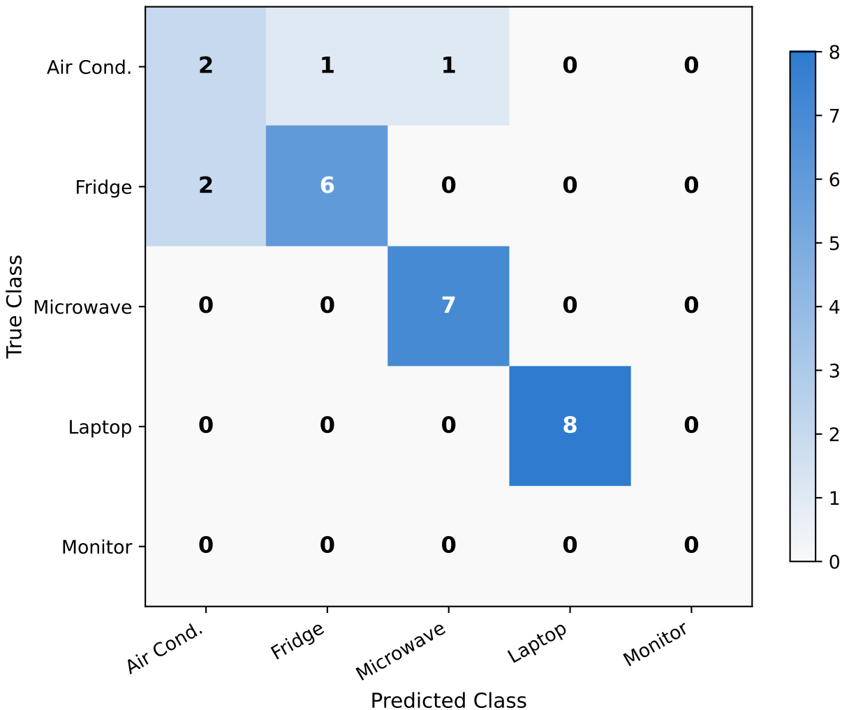
Figure 5.2a — Classification Confusion Matrix (Roboflow RF-DETR Custom Model)
