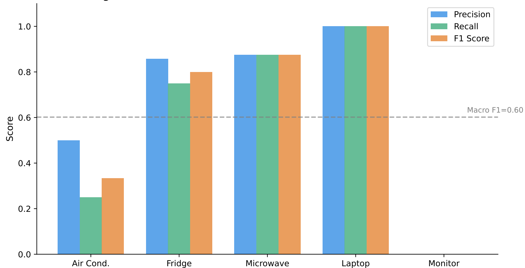
Figure 5.2b — Per-Class Detection Metrics (Roboflow RF-DETR)
