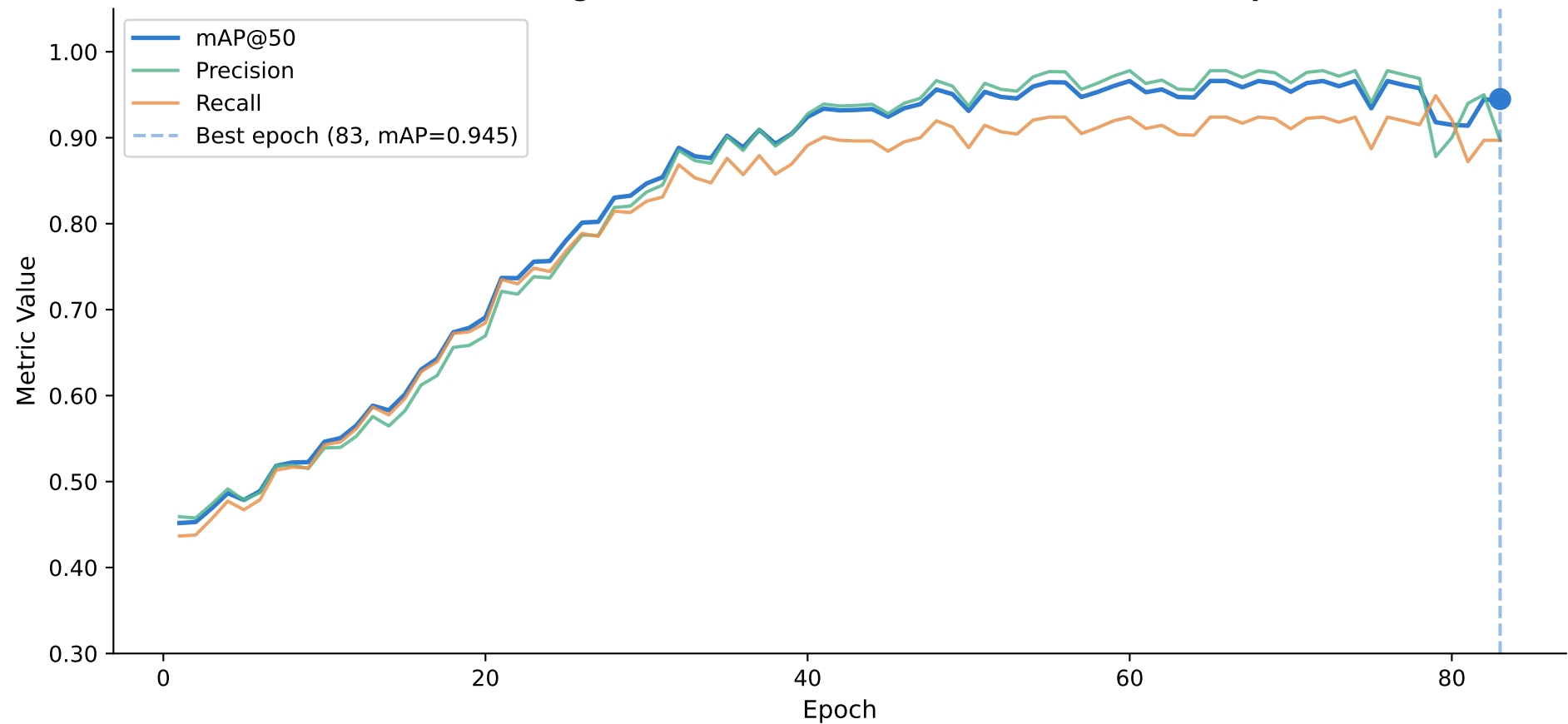
YOLOv5s Training Curves — Run v2 (Extended Fine-Tune, 83 Epochs)
