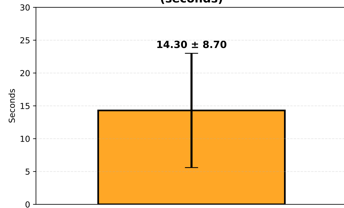
Runtime (seconds)
