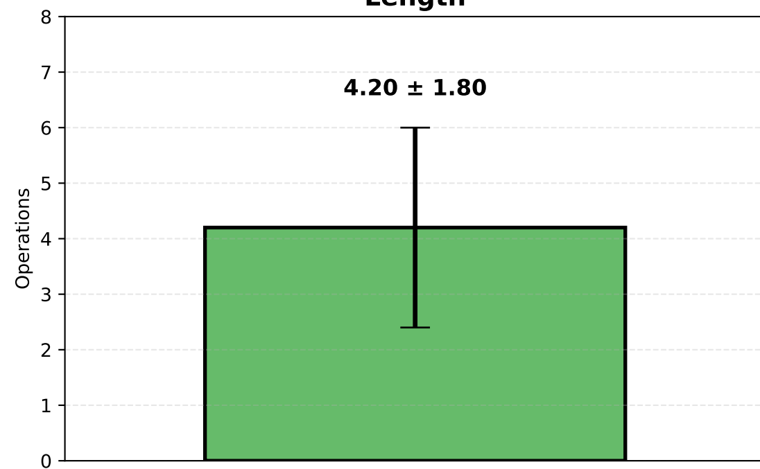
Program Length
