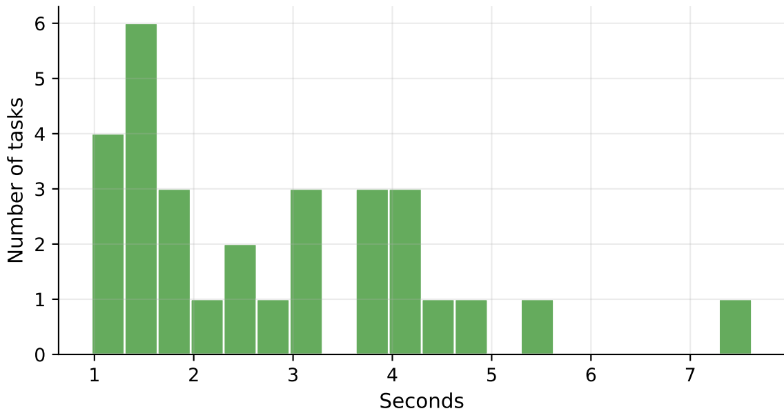
Per-Task Runtime Distribution (seconds)
