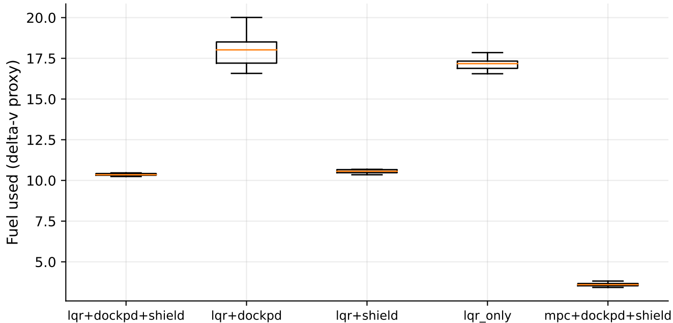
Spacecraft Rendezvous: Fuel Usage Distribution (20 seeds)
