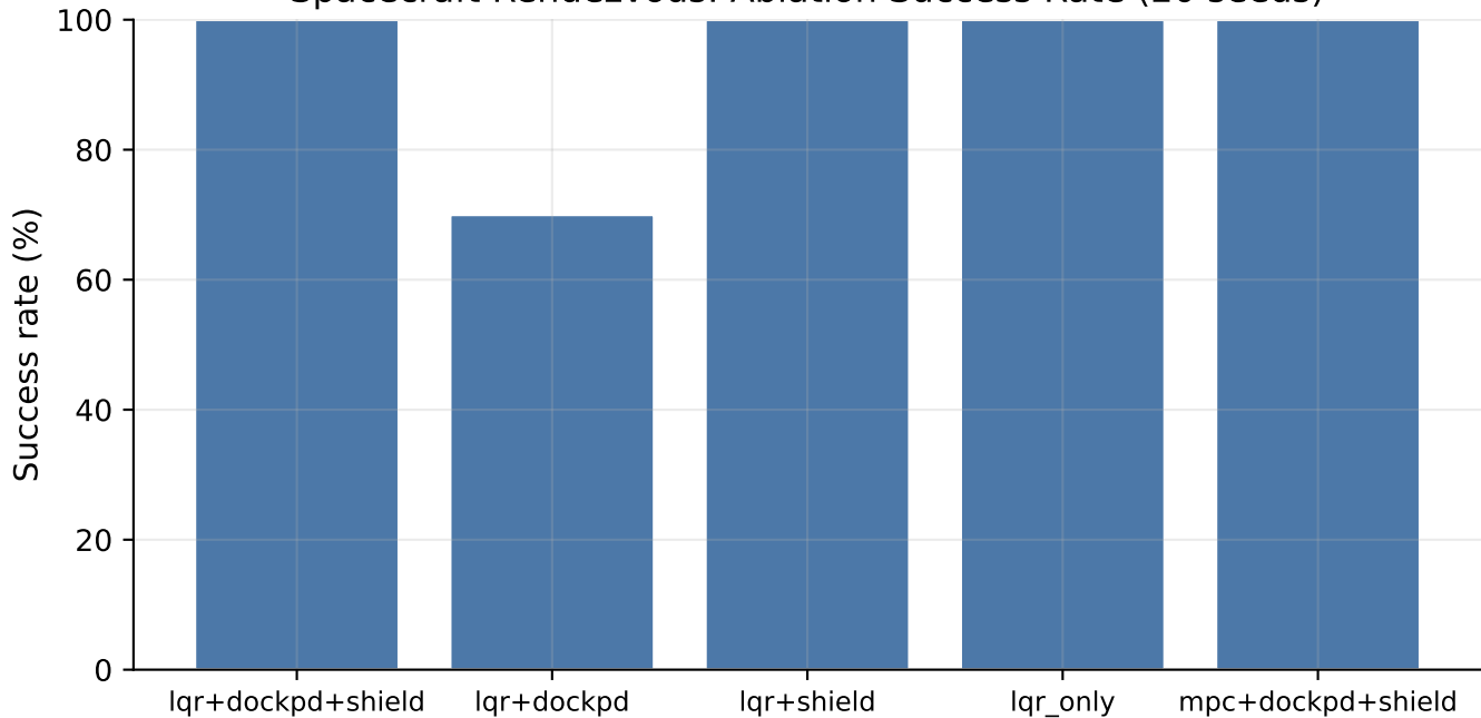
Spacecraft Rendezvous: Ablation Success Rate (20 seeds)
