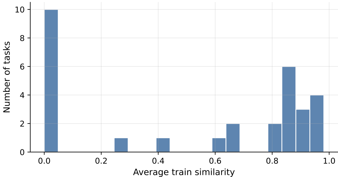
SMPMA: Train Similarity Score Distribution (Evaluation Set)
