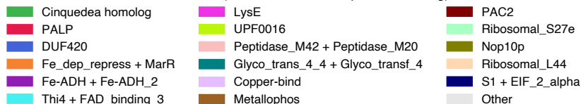
Gene families ( \pm 5 kb around the cinquedea homolog)
