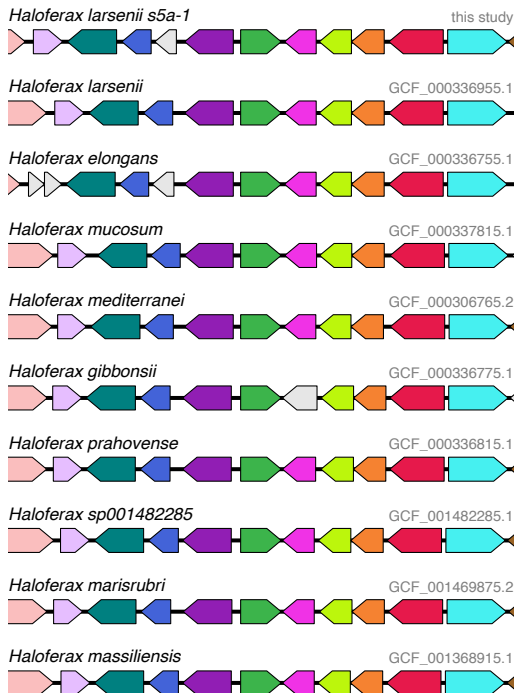
Gene families ( \pm 5 kb around the cinquedea homolog)
