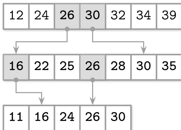
Figure 6-5. Fractional cascading
