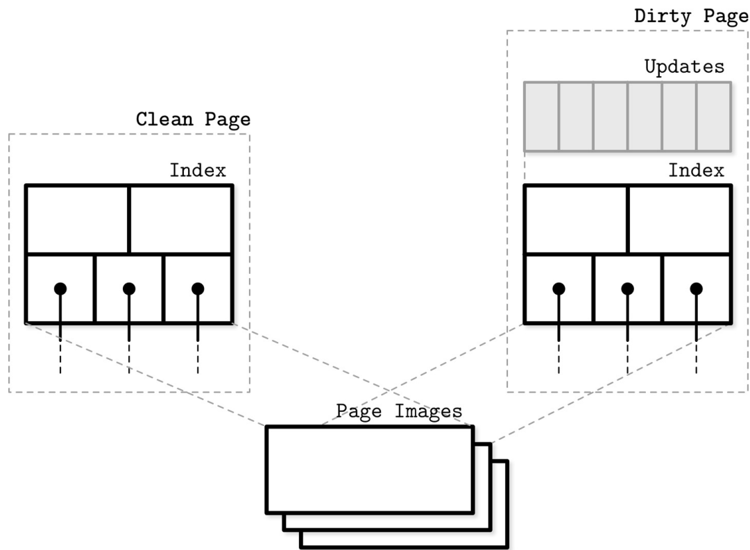
Figure 6-3. WiredTiger pages
