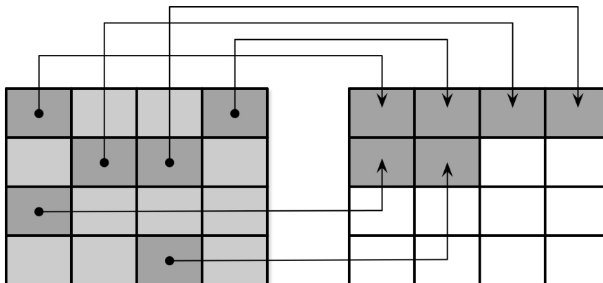
Figure 7-14. Page relocation during garbage collection
