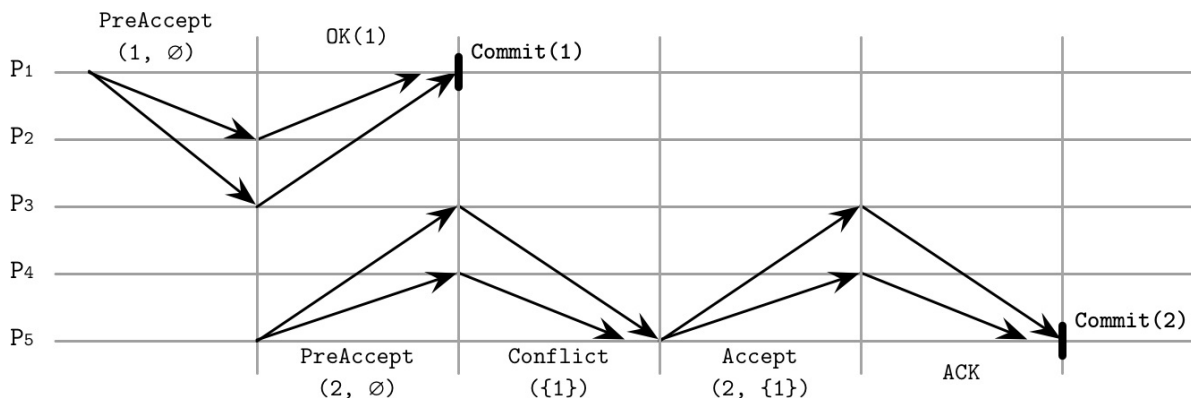
Figure 14-8. EPaxos algorithm run
