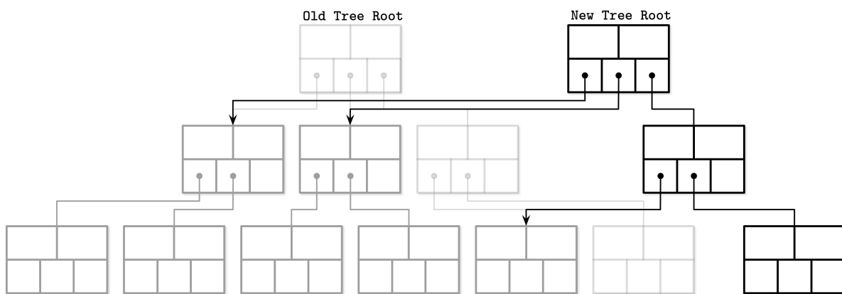
Figure 6-1. Copy-on-write B-Trees
