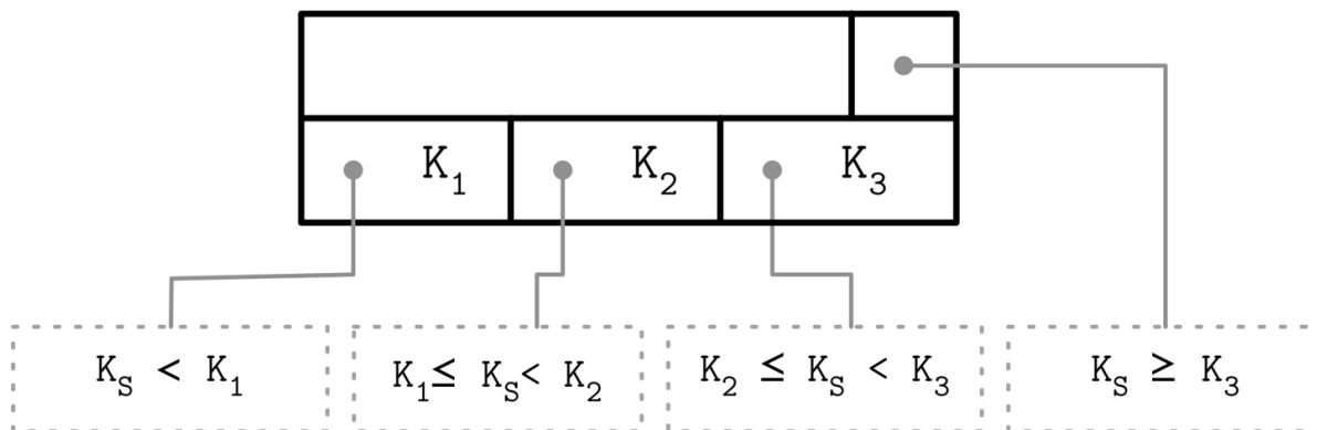
Figure 4-2. Rightmost pointer
