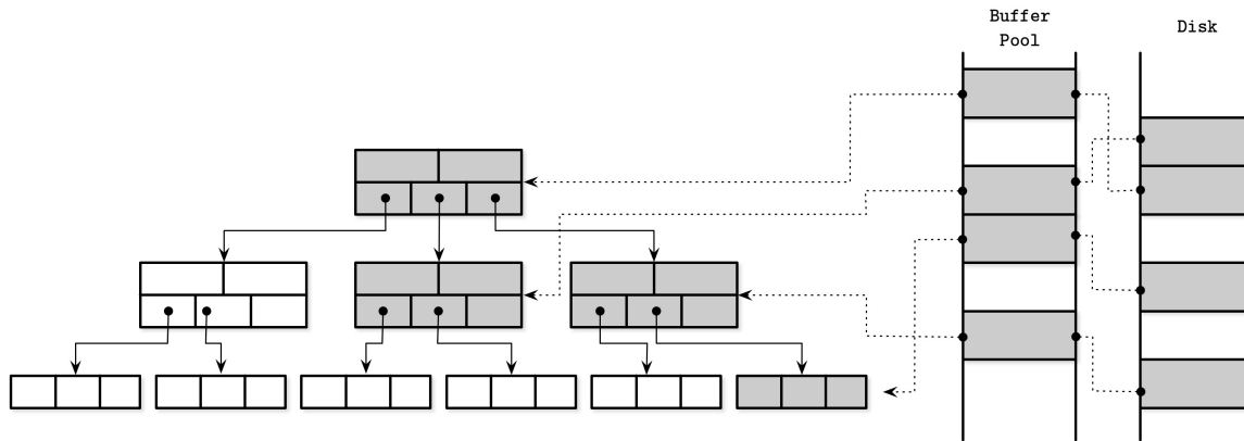
Figure 5-1. Page cache
