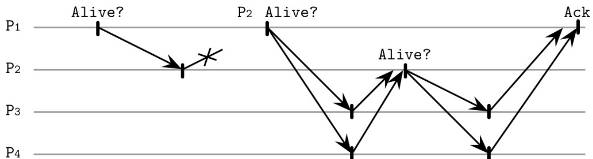
Figure 9-3. "Outsourcing" heartbeats
