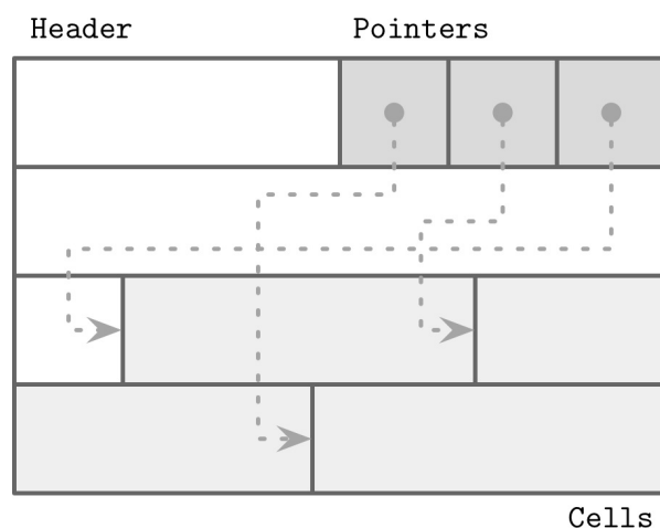
Figure 3-5. Slotted page
