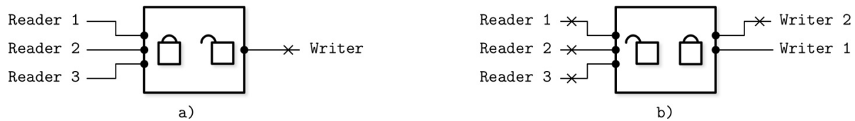
Figure 5-8. Readers-writer locks
