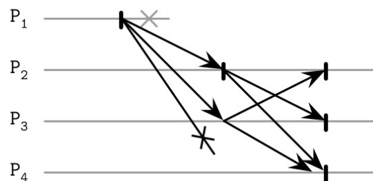
Figure 14-1. Broadcast
