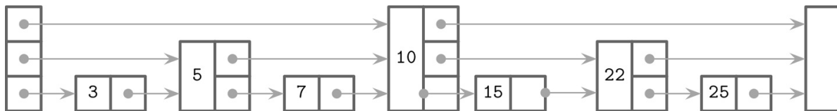
Figure 7-8. Skiplist
