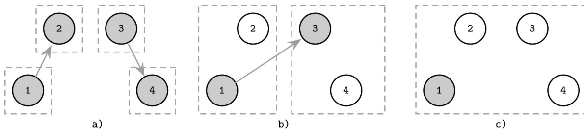
Figure 10-4. Invitation algorithm
