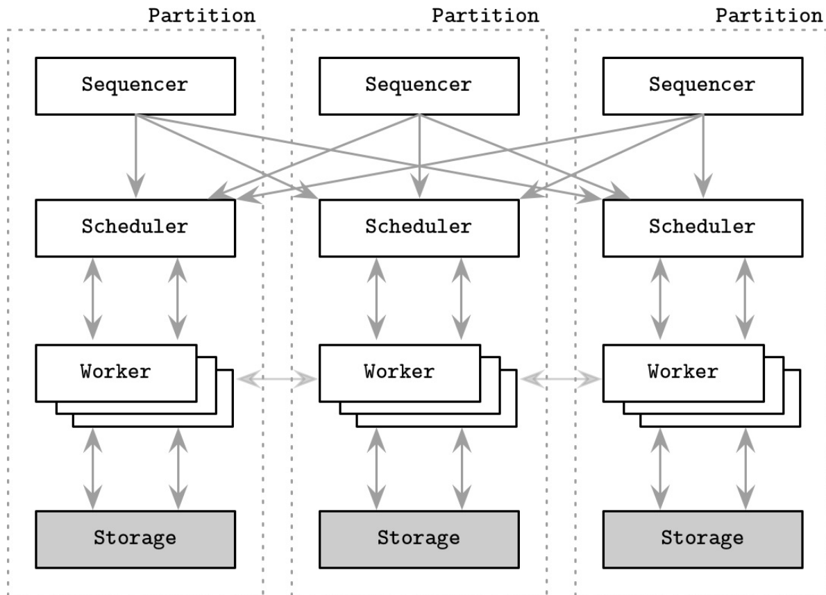
Figure 13-7. Calvin architecture
