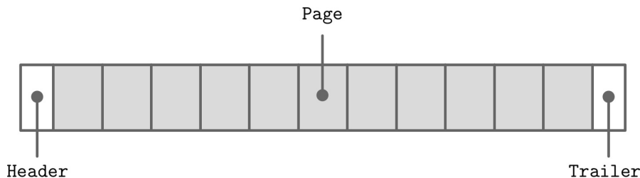
Figure 3-3. File organization
