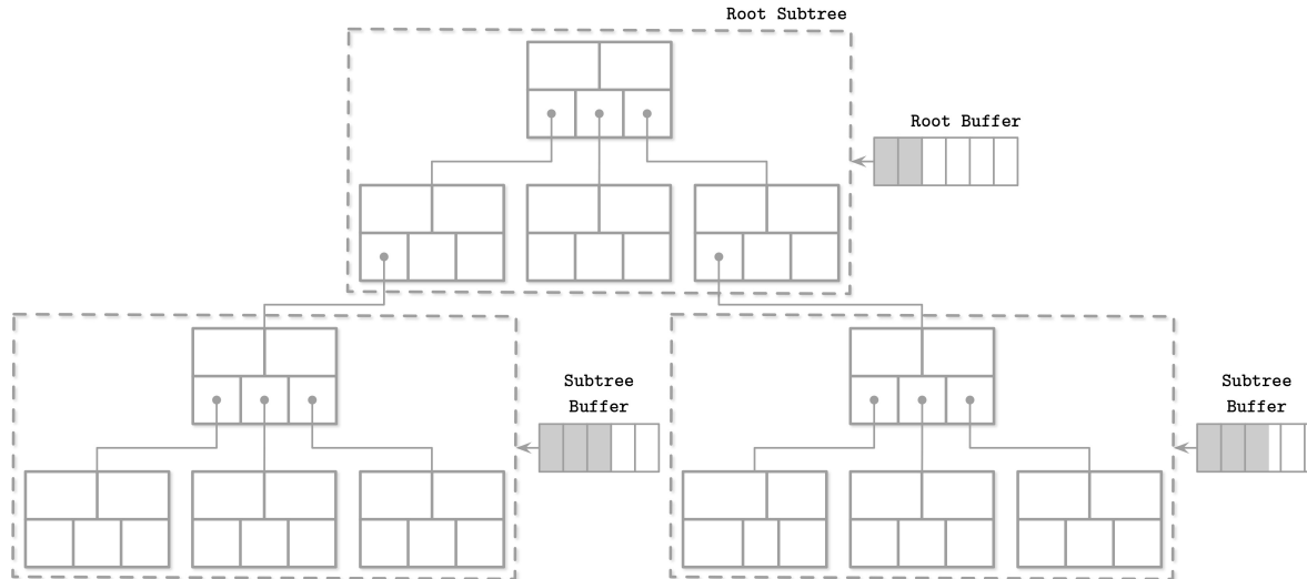
Figure 6-4. LA-Tree
