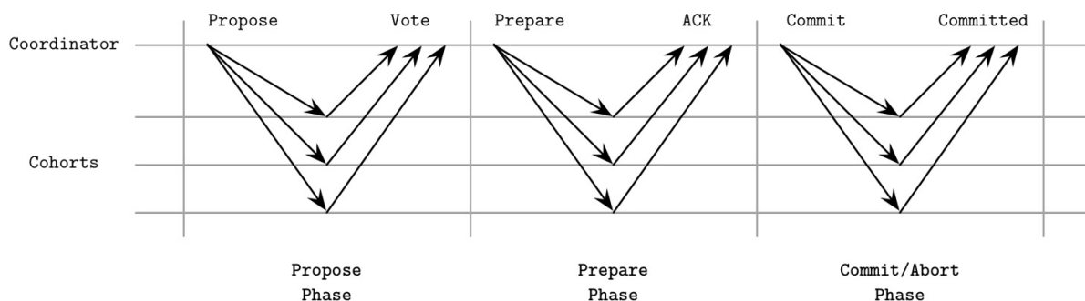
Figure 13-5. Three-phase commit
