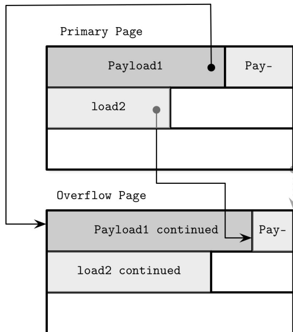
Figure 4-6. Overflow pages
