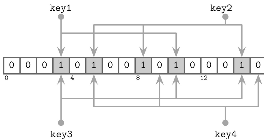
Figure 7-7. Bloom filter
