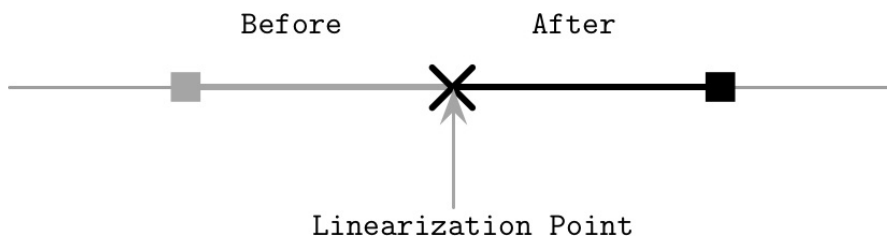
Figure 11-4. Linearization point
