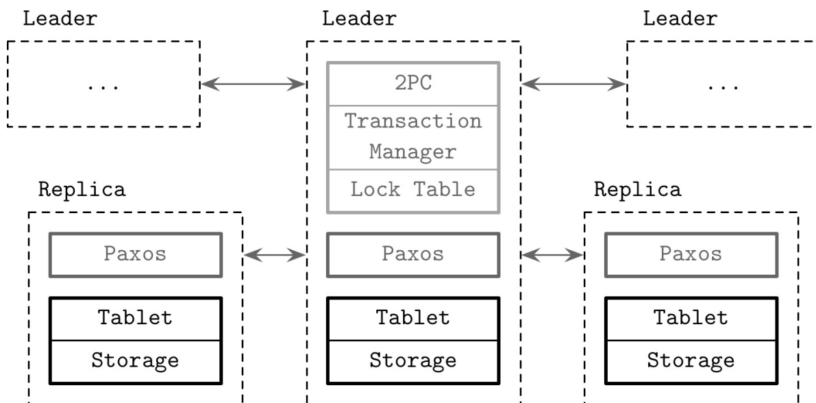
Figure 13-8. Spanner architecture
