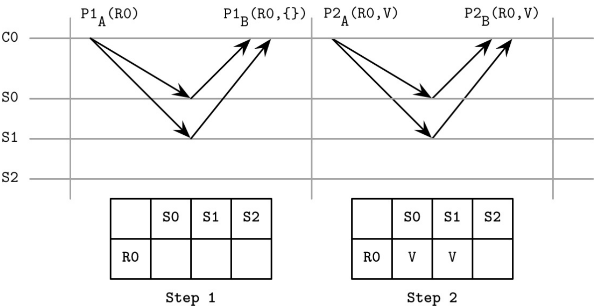
Figure 14-9. Generalization of Paxos
