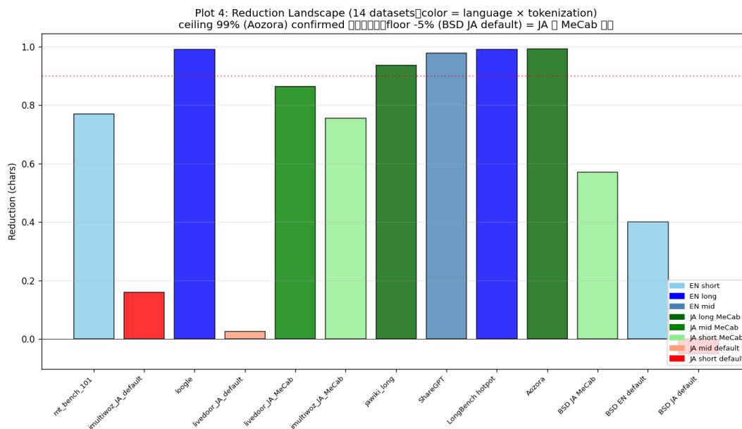
Plot 4. Reduction landscape across 14 datasets (= main paper Figure 2). Colored by language × tokenization.
