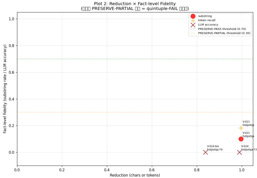
Plot 2. Reduction × fact-level fidelity. All measured points cluster in PRESERVE-FAIL region ( \leq 0.30 threshold), visualizing the quintuple-FAIL constitutive limit.
