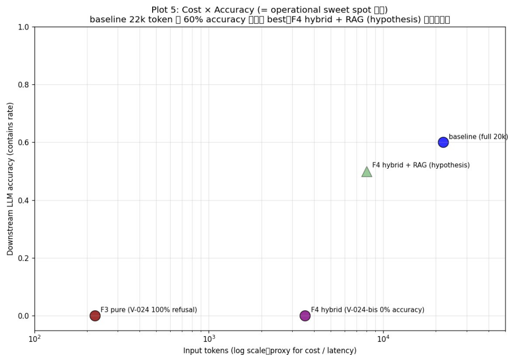
Plot 5. Cost × downstream LLM accuracy (= main paper Figure 4). F4 hybrid + RAG hypothesis intersection marked.
