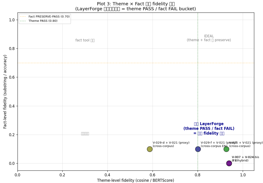
Plot 3. Theme × fact two-layer structure (= main paper Figure 1). LayerForge variants in lower-right quadrant (theme PASS / fact FAIL).
