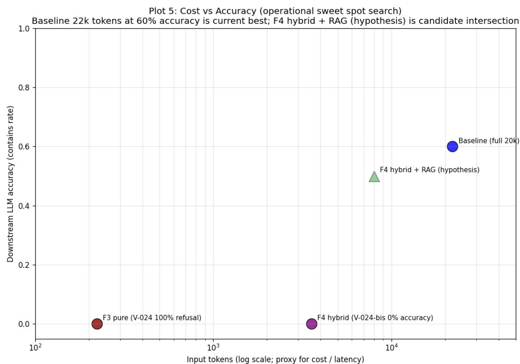
Plot 5. Per-query input-token cost vs downstream LLM accuracy (= main paper Figure 4; see main Figure 4 caption for full details). Raw data: v029a_cost_latency_results.json.
