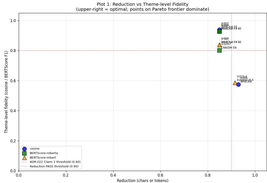
Plot 1. Reduction vs theme-level fidelity Pareto frontier (= main paper Figure 3).
