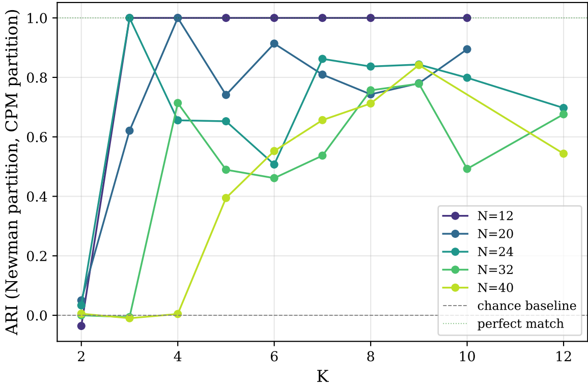
Partition agreement between methods, by corpus size N
