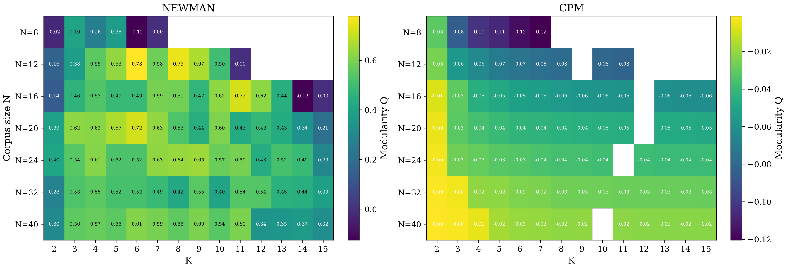
Modularity Q heatmap: N \times K — Newman vs CPM (cross-domain mpnet)
