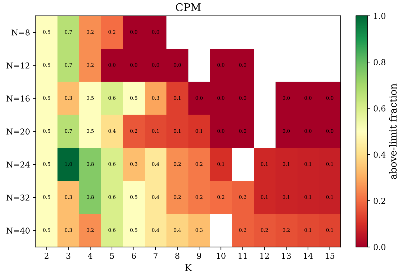
Above-limit fraction (Fortunato-Barthélemy): N \times K — Newman vs CPM
