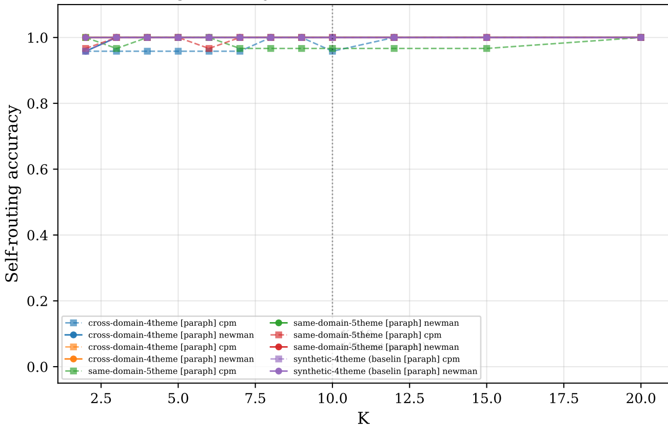
Self-routing accuracy vs K — Newman (solid) vs CPM (dashed)
