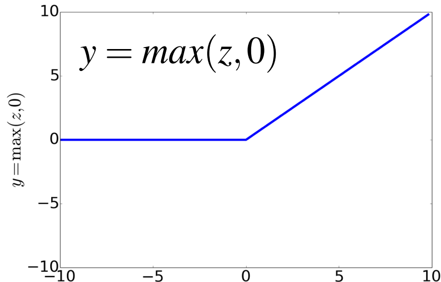
ReLU
