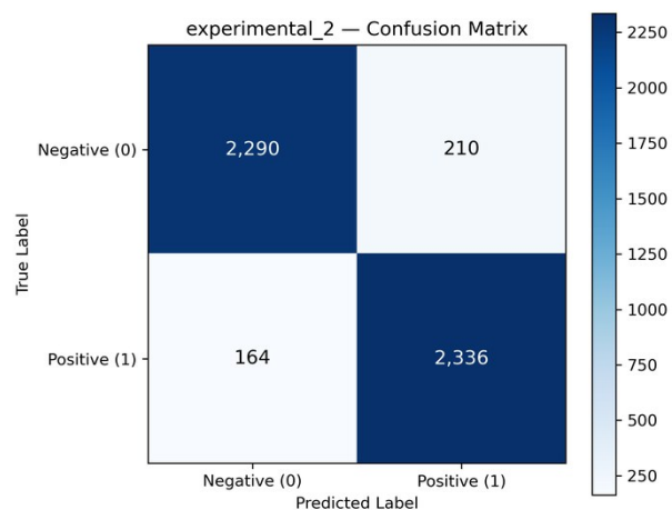
Aswin TextCNN confusion matrix: TN 2,290; FP 210; FN 164; TP 2,336.
