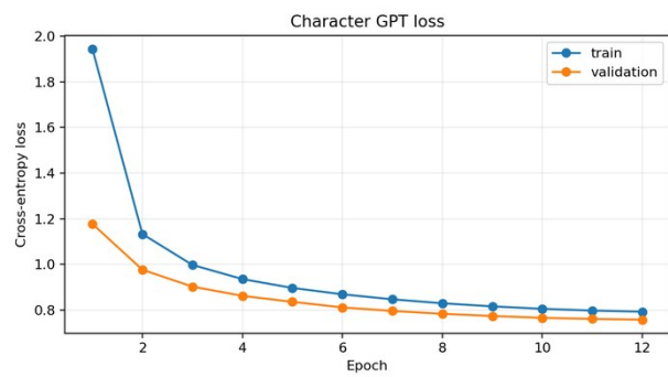
Aswin: loss falls through epoch 12. The lower validation curve reflects dropout being disabled during validation, not leakage.
