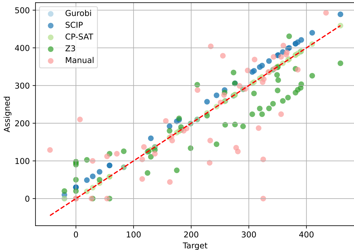
Assigned vs Target 2022-GUROBI-SCIP-SAT-Z3
