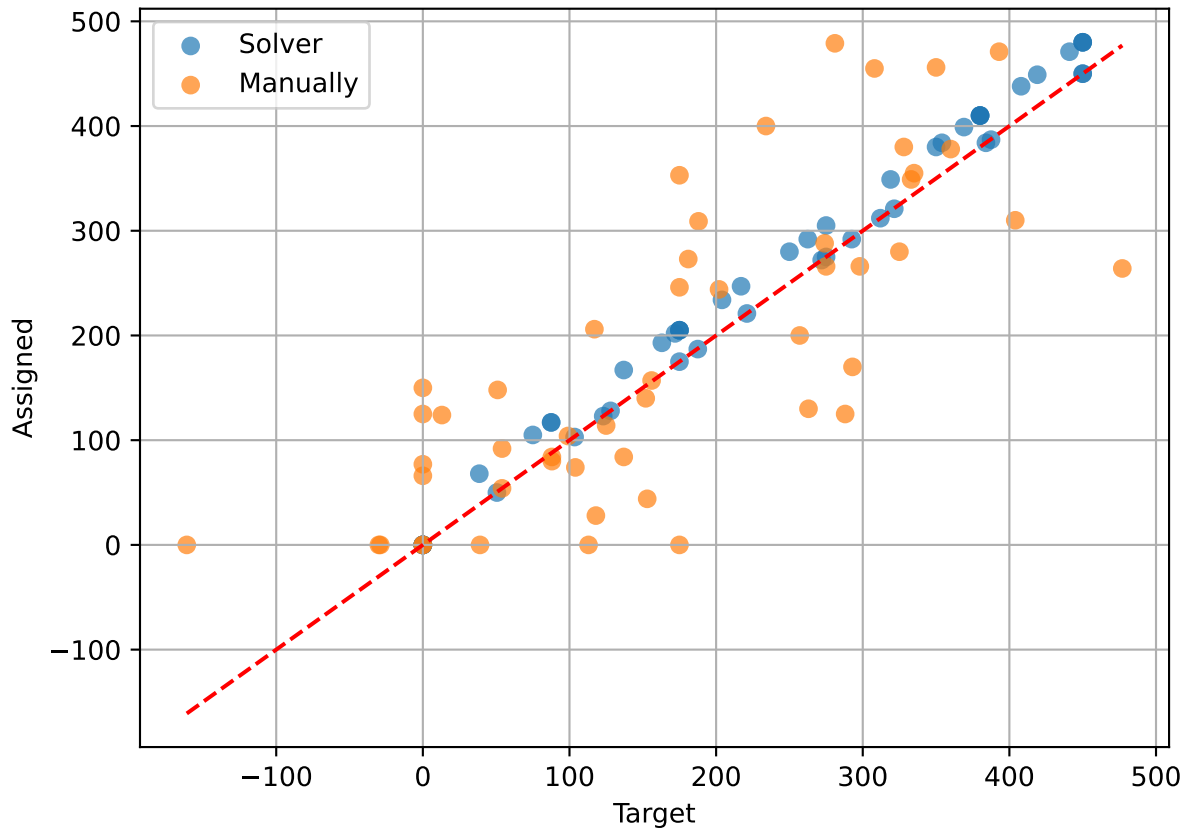
Assigned vs Target 2023-GUROBI
