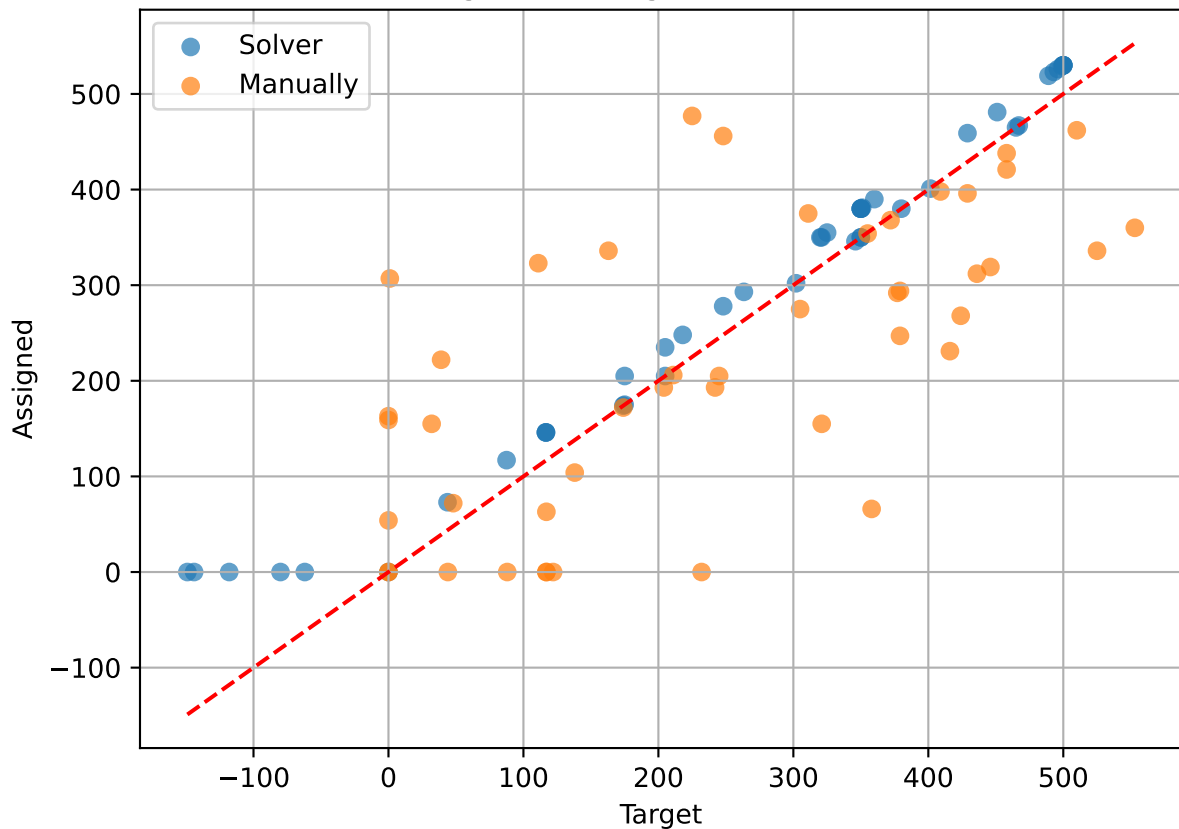
Assigned vs Target 2025-GUROBI
