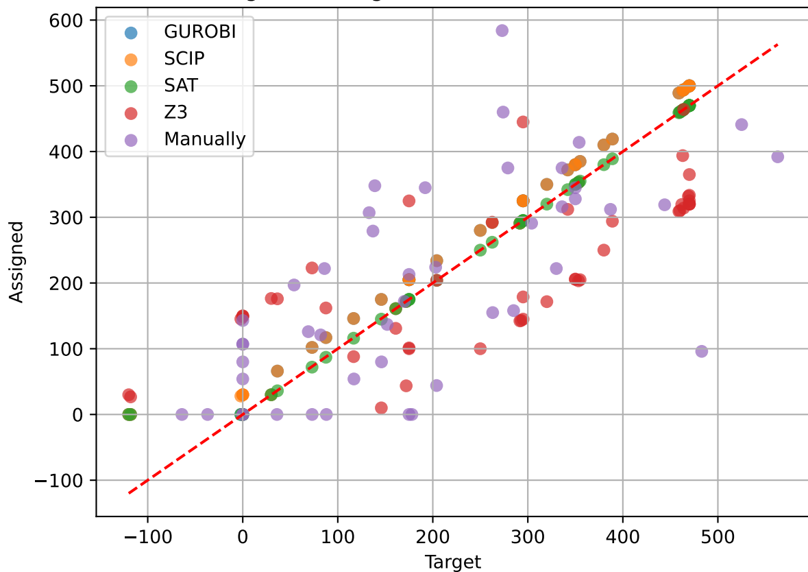
Assigned vs Target 2024-GUROBI-SCIP-SAT-Z3
