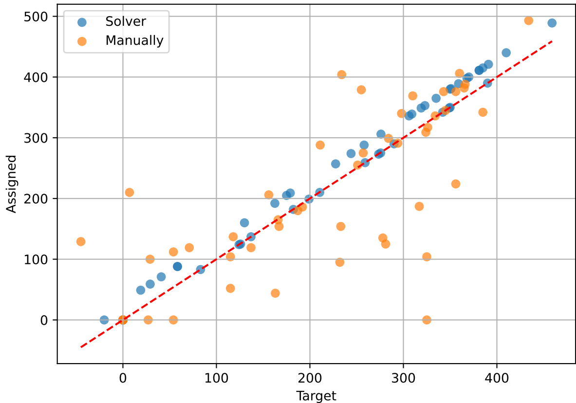
Assigned vs Target 2022-GUROBI
