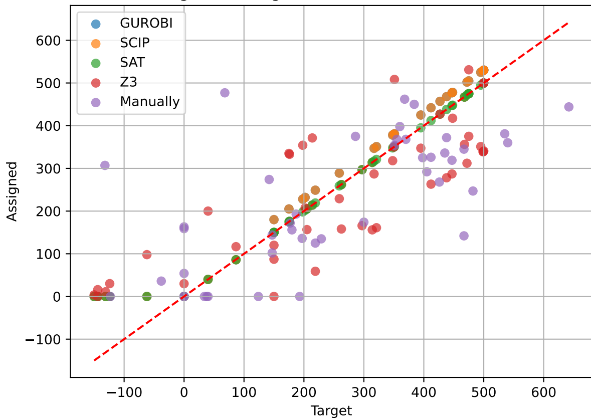
Assigned vs Target 2026-GUROBI-SCIP-SAT-Z3
