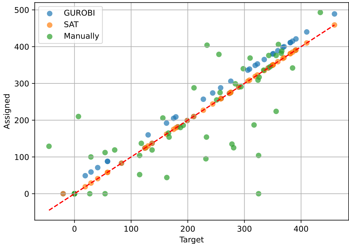
Assigned vs Target 2022-GUROBI-SAT
