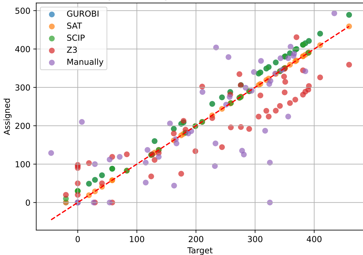
Assigned vs Target 2022-GUROBI-SAT-SCIP-Z3
