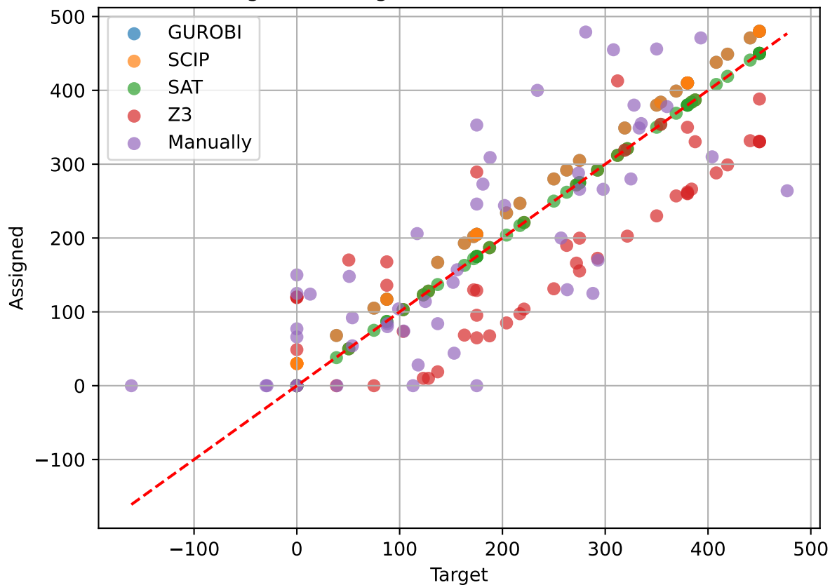
Assigned vs Target 2023-GUROBI-SCIP-SAT-Z3
