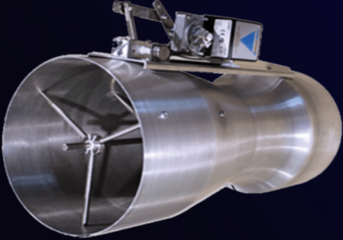
Air Venturi Valves
