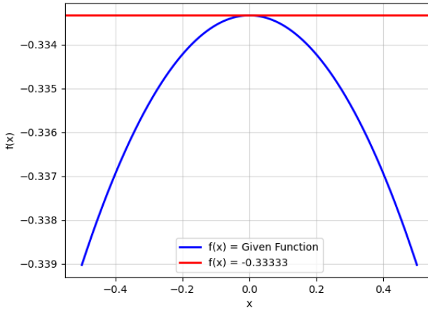
Fig. 1.2.7.1. The plot depicting the approaching of the limit to \frac{-1}{3}
