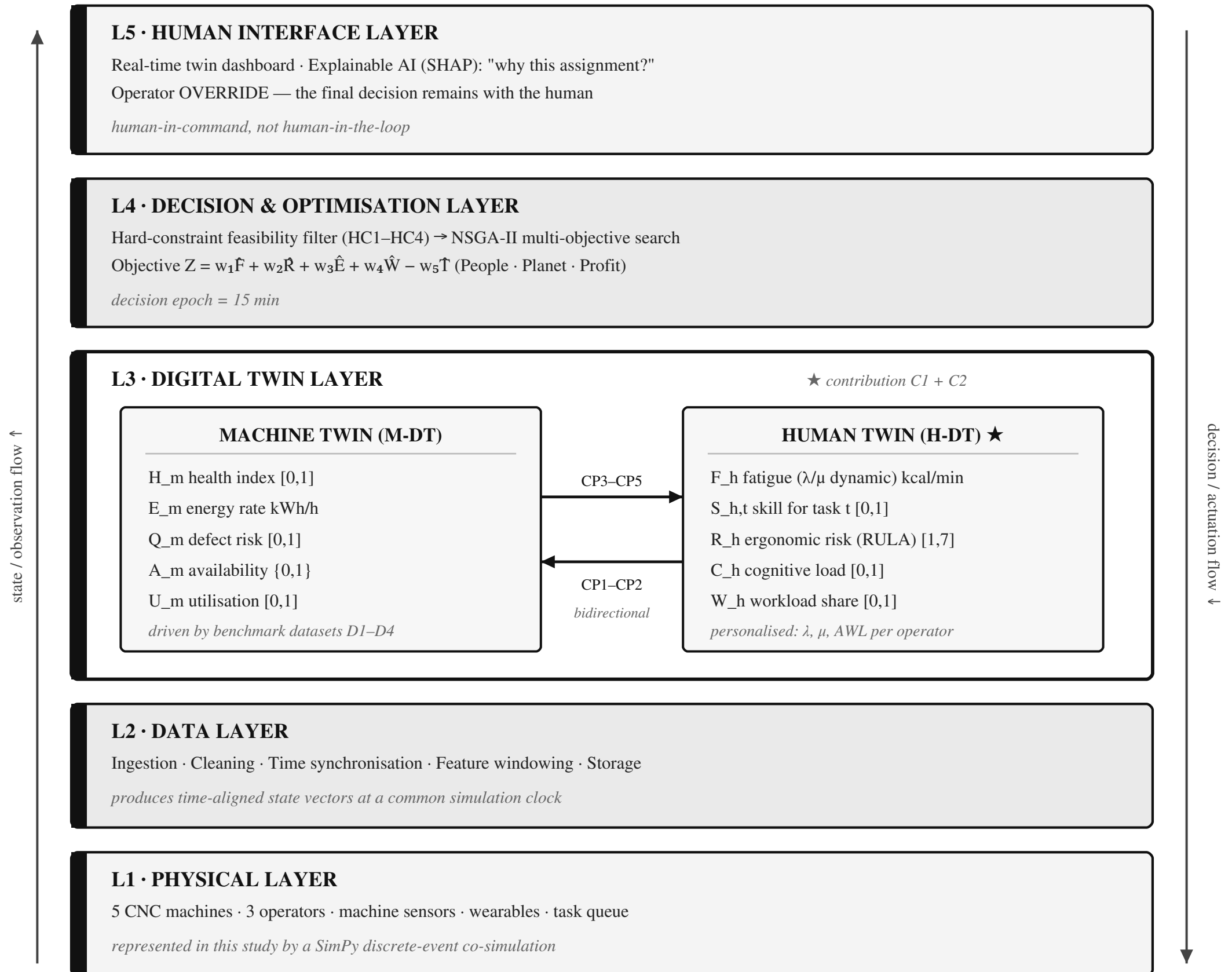
Fig. 1. Five-layer reference architecture. The novelty is L3: a machine twin and a quantified, personalised human twin exchanging state bidirectionally, both feeding a single constrained multi-objective decision layer.
