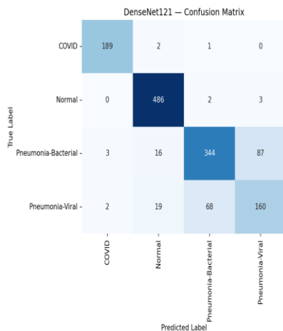
Figure 6.1a: DenseNet121 confusion matrix.
