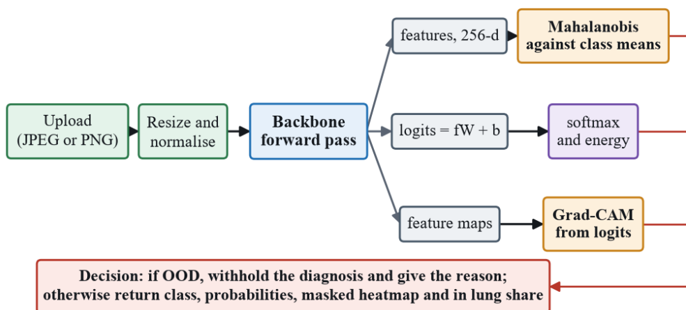
Figure 5.1: Inference pipeline block diagram, showing the single forward pass from which the classification, the validity verdict and the explanation are all derived.
