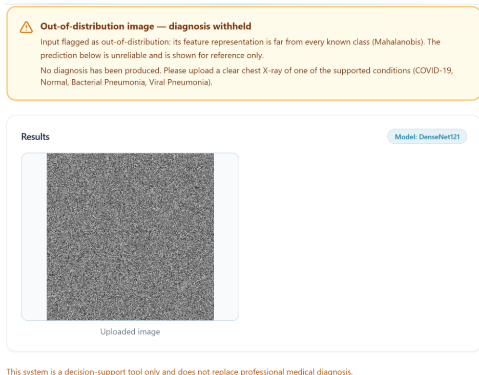
Figure 5.2: Execution evidence for FR4. The analysis view of the running platform after a synthetic noise image was submitted, showing the withheld diagnosis and the reason in place of any diagnostic content.
