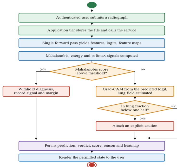
Figure 4.3: Activity diagram of the analysis workflow.
