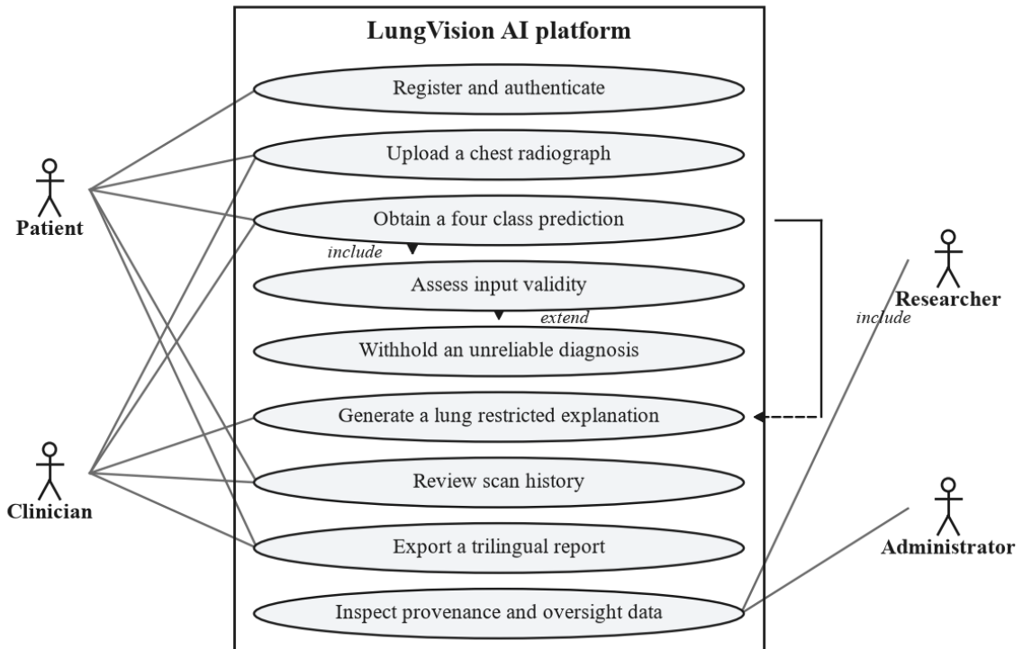
Figure 4.1: Use case diagram of the delivered platform.
