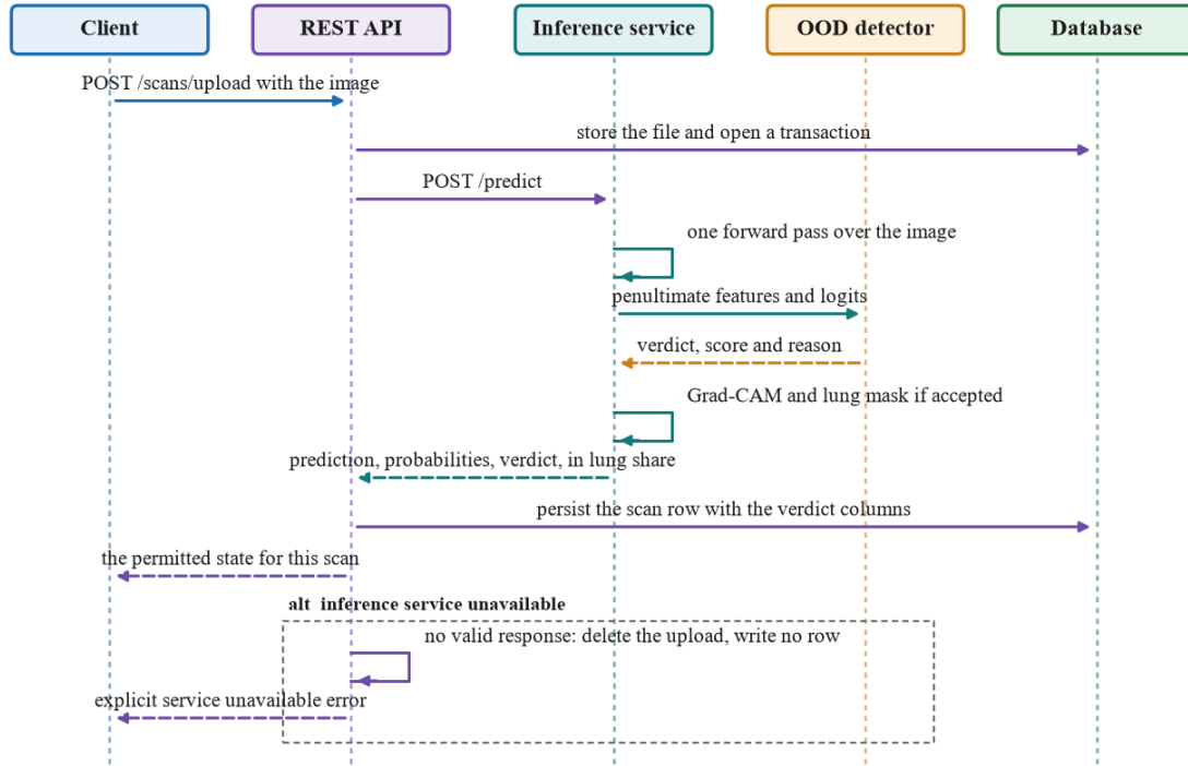
Figure 4.4: Sequence diagram for the upload and analyse use case.
