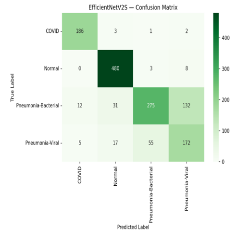
Figure 6.1c: EfficientNetV2S confusion matrix.
