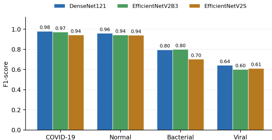
Figure 6.2: Per class F1 for the three architectures, showing a consistent difficulty ordering across models.
