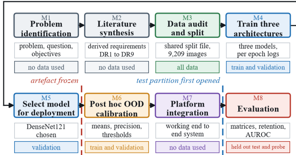
Figure 3.1: Research methodology execution workflow, showing the order of the phases and the point at which the artefact was frozen for evaluation.
