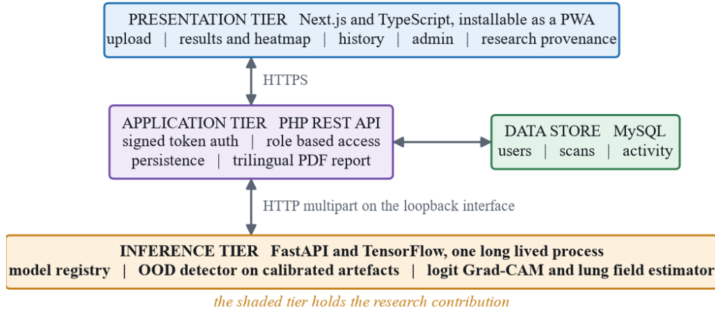
Figure 4.5: Proposed deployment architecture, showing the three tiers, the data store and the location of the research contribution.
