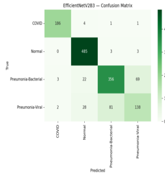
Figure 5.2: EfficientNetV2B3 confusion matrix.
