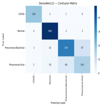
Figure 5.1: DenseNet121 confusion matrix.
