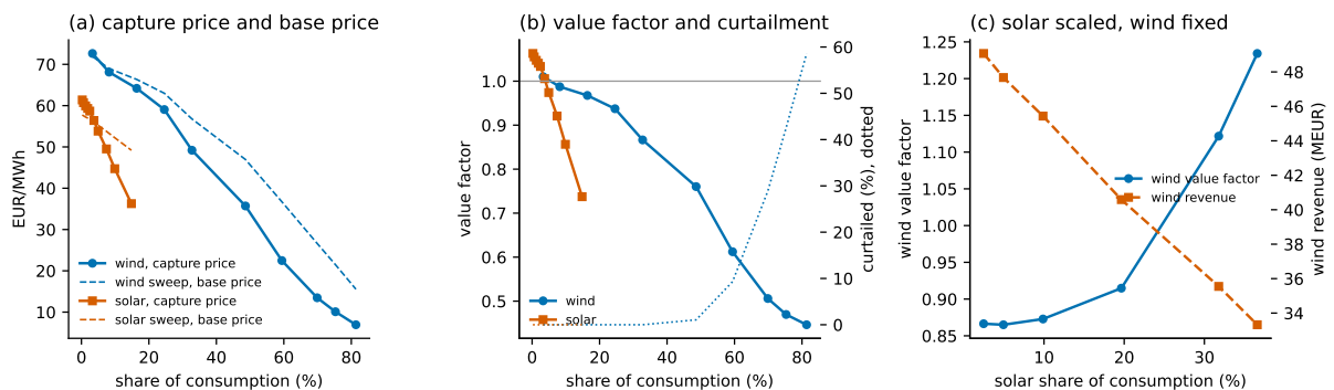
Figure 1: The same numbers. (a) capture price against the technology's own share, base price along the same sweep dashed; (b) value factor, with curtailment dotted on the right axis; (c) solar scaled while wind is fixed: wind's value factor and wind's revenue.
