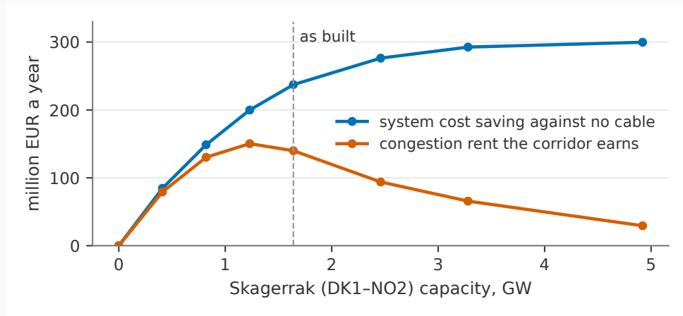
Energy System Models, Fig. 6.8, redrawn: the Skagerrak swept from zero to three times its size, 2024. Gross of the cable's cost.
