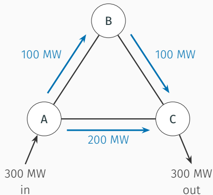
Energy System Models, Fig. 6.3, redrawn: 300 MW from A to C over three identical AC lines.
