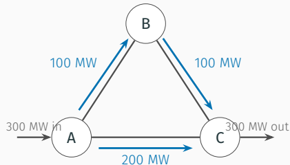
Energy System Models, Fig. 6.3: 300 MW from A to C over three identical AC lines.
