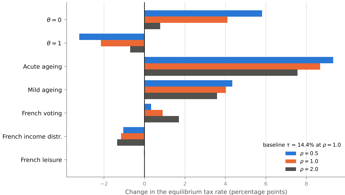
Effect of each counterfactual on the equilibrium tax rate
