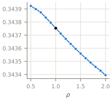
Productivity \eta_0
