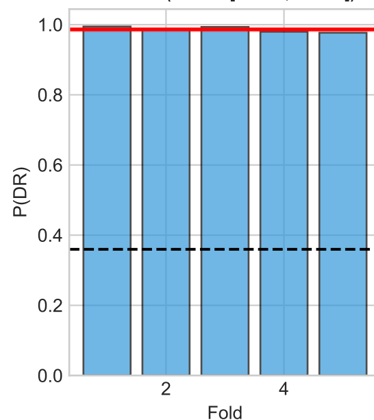
Per-Fold (95% CI [0.9800, 0.9926])
