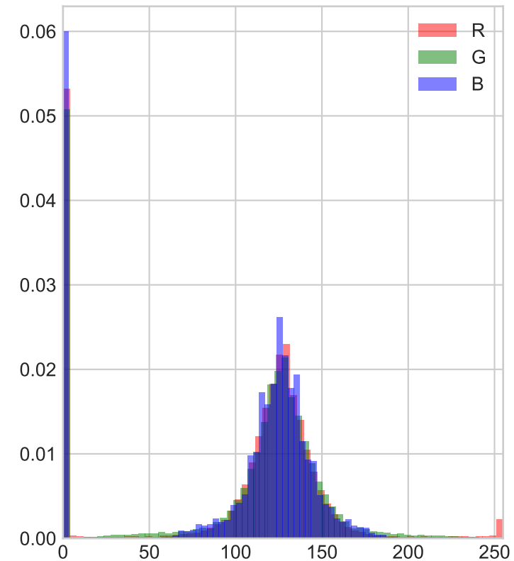
Preprocessed Histograms
