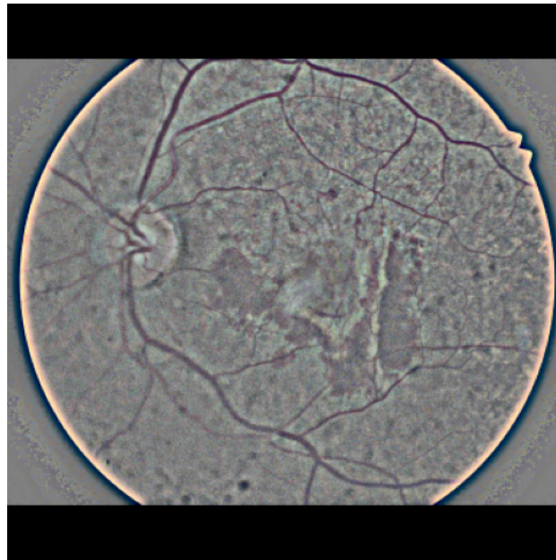
Step 5: Final (384×384)
