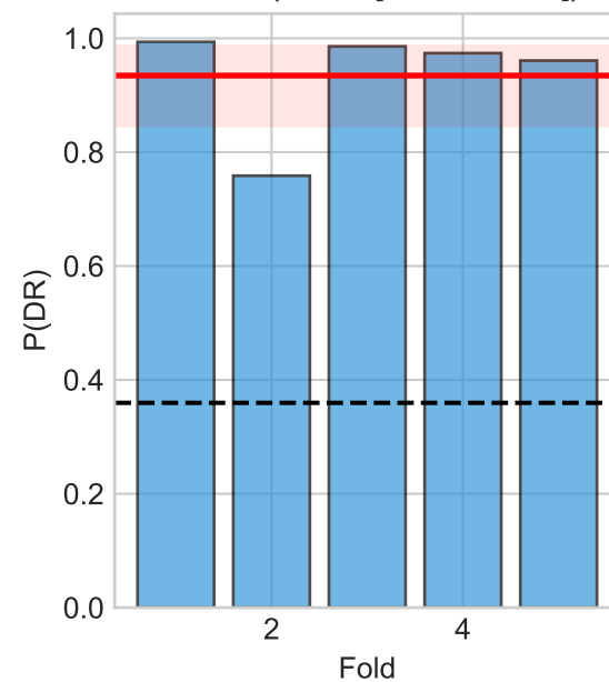
Per-Fold (95% CI [0.8460, 0.9865])
