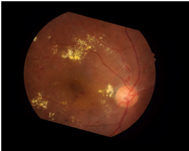
Step 1: Original
