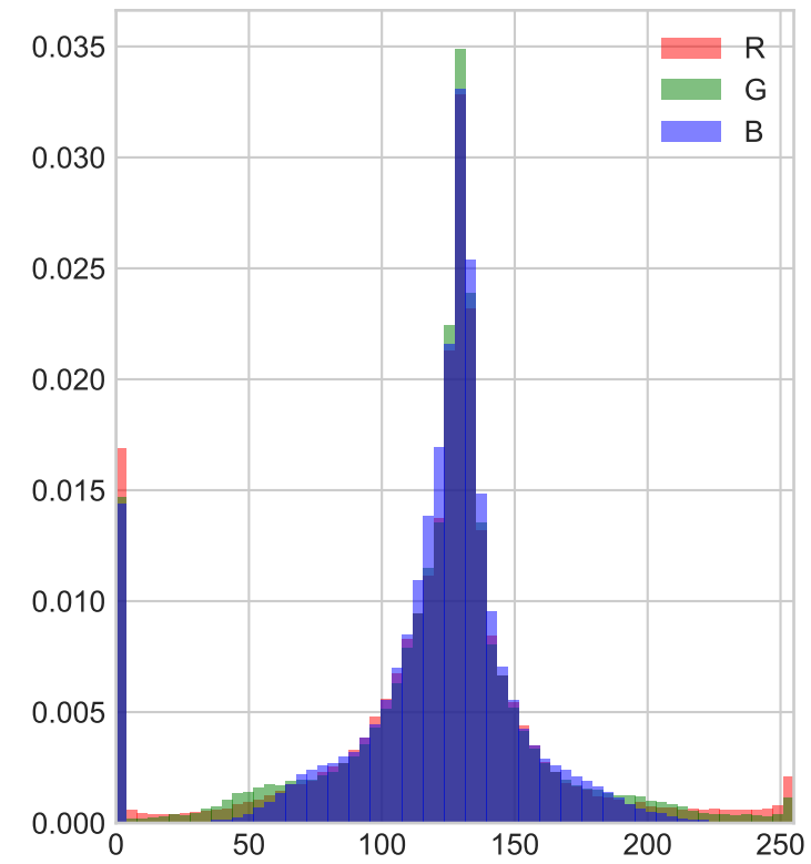
Preprocessed Histograms
