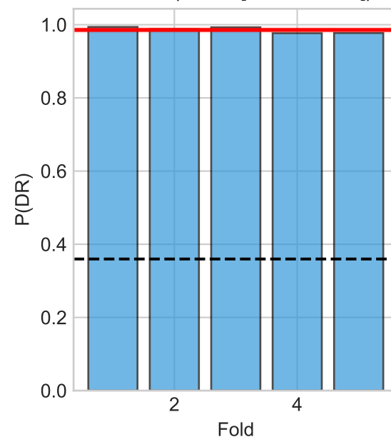
Per-Fold (95% CI [0.9792, 0.9923])
