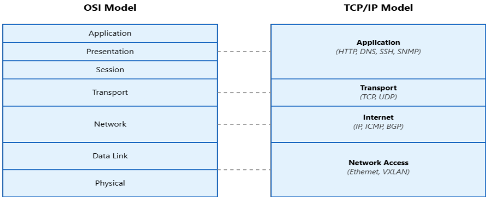
Figure 2.5: OSI vs TCP/IP Layering Models
