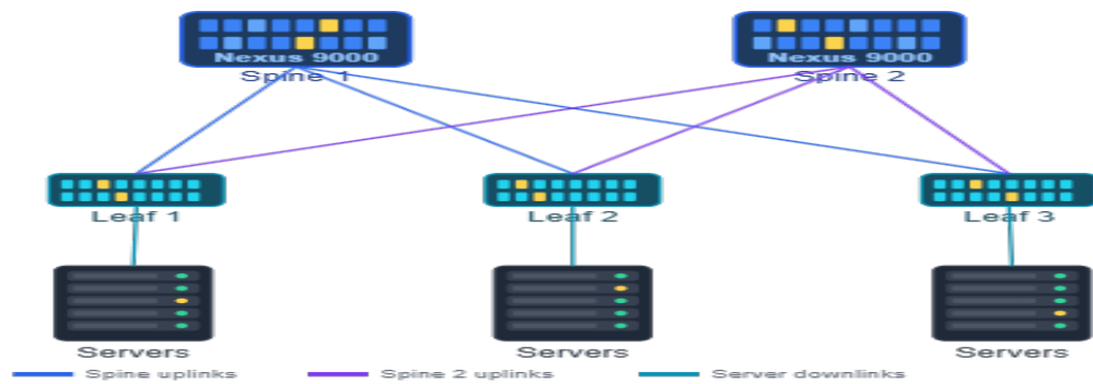
Figure 2.7: Spine-Leaf Topology
