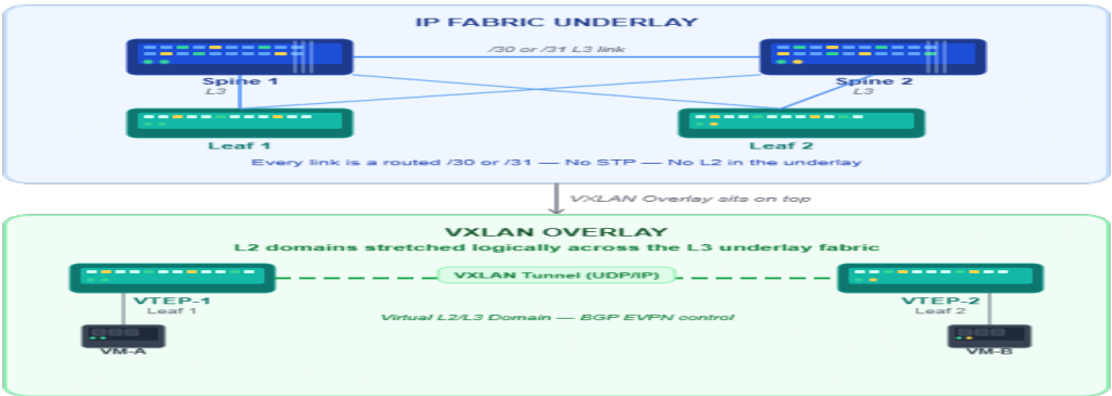
Figure 2.9: Underlay vs Overlay Diagram
