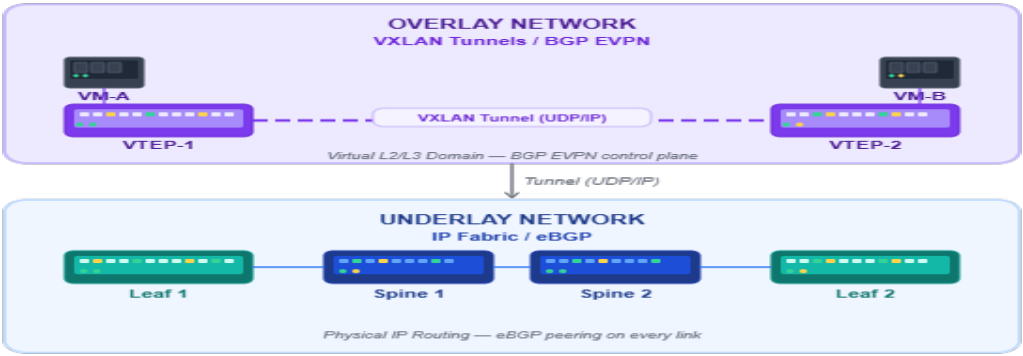
Figure 2.8: IP Fabric Underlay Concept
