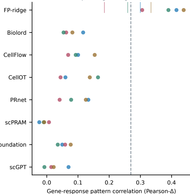
a Expression-pattern fidelity
