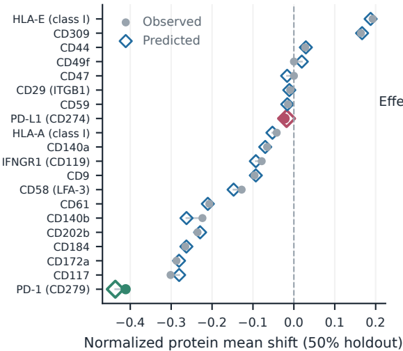
c Program and transcriptome agreement
