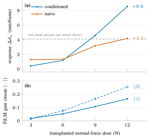
Fig. 4. On-robot counterfactuals (P5): identical frozen observations, wrench transplanted to a fixed normal-force dose. (a) The response ordering reverses between 6 and 9 N—the offline crossover on the physical system. (b) FiLM modulation magnitude rises monotonically with dose.
